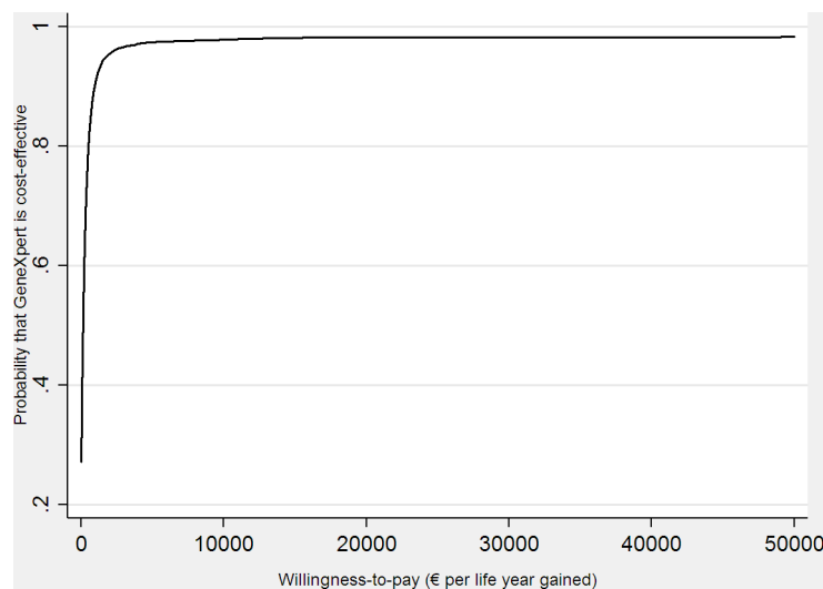
Fig 3. The probabilistic sensitivity analysis.
