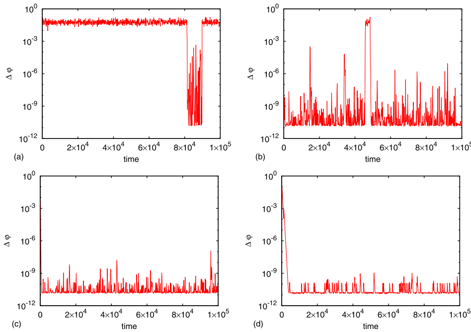
FIG. 1. Time evolution of the synchronization error \Delta\phi(t) for different \tau_p . All results are for d=32 . (a) \tau_p = 1 , where the system is not synchronized ( \Delta\phi \sim 10^{-1} ), but sometimes the synchronization error can be very small. (b) \tau_p = 3 . The synchronized state lasts longer than (a). (c) \tau_p = 11 , and (d) \tau_p = 100 . After the initial transient, synchronization is achieved. The noise is not strong enough to break the synchronized state. Note that the FSA (see Sec. IV A) describes the dynamics leading to the synchronization for these cases.
