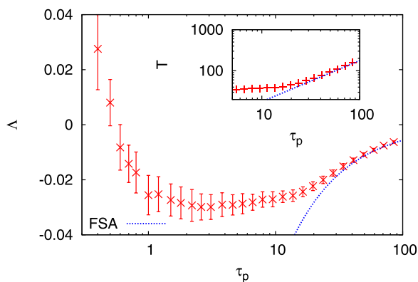
FIG. 4. Transverse Lyapunov exponent \Lambda for d=30 . Blue line represents the prediction of the fast switching approximation (8). In the inset, the characteristic time T = 1/|\Lambda| is shown in a log-log scale. The average is taken over 124 realizations.
