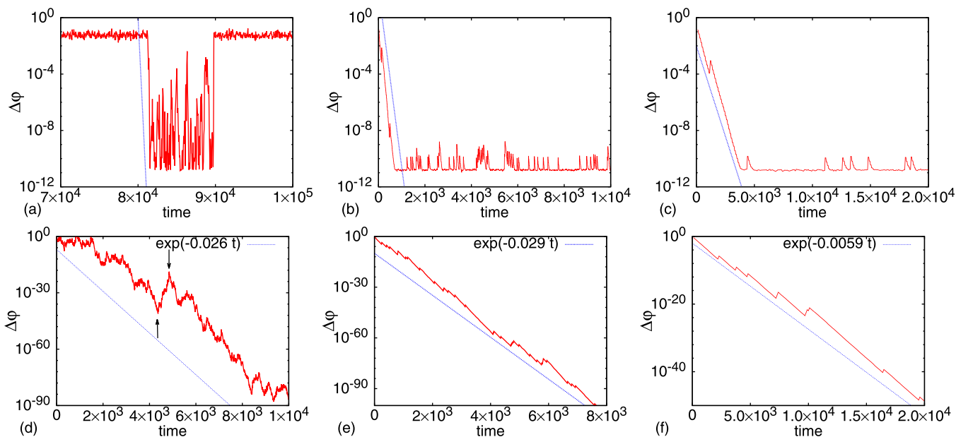
FIG. 3. Comparison of the time evolution of the synchronization error for the original nonlinear equation (2) versus the linearized equation (6) for \tau_p = 1 (a) and (d), \tau_p = 11 (b) and (e), and \tau_p = 100 (c) and (f). Upper panels are close-up of Fig. 1 for the corresponding parameter values from the nonlinear equation. Lower panels represent the results of the linearized equation for the same parameter values to the upper panels. The slope of the blue lines corresponds to the transverse Lyapunov exponent \Lambda . In panel (d), although \Lambda is negative, its fluctuation is so large that \Delta\phi can grow temporarily. The arrows indicate such an example of the temporal growth of \Delta\phi .
