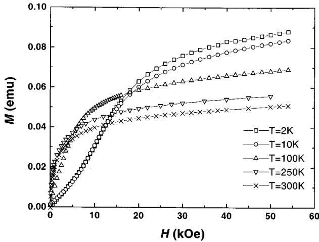
FIG. 4. Magnetization vs applied magnetic fields obtained at different sample temperatures.
