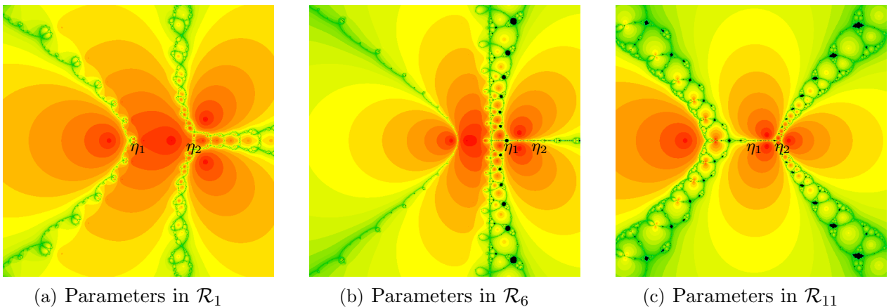
FIGURE 4. Dynamical planes for parameters in \mathcal{R}_1 , \mathcal{R}_6 and \mathcal{R}_{11} . In all three cases the Fatou set is different from the union of all the basin of attraction of the roots of p .
