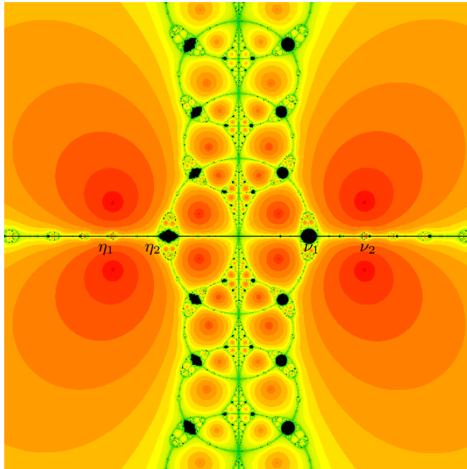
FIGURE 1. Dynamical plane of N_{a,b} for a = 0.0013 and b = -1.73729 in the region \mathcal{R}_4 . We can see in red the four basins of attractions of the complex roots of p_{a,b} and in black the two attracting cycles of period two, \{\eta_1, \eta_2\} and \{\nu_1, \nu_2\} , to which the free critical points are attracted.
