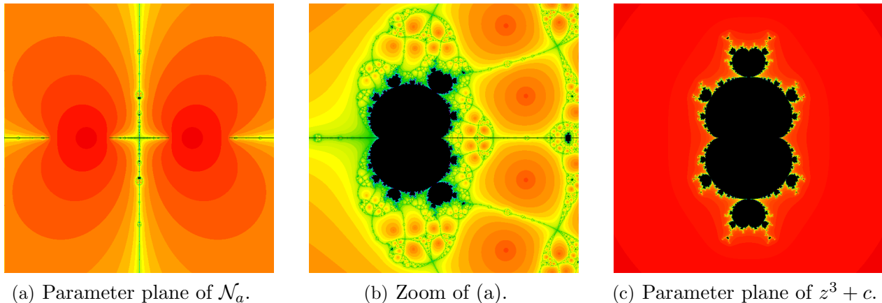
FIGURE 5. The parameter plane of \mathcal{N}_a for complex values of a (figures (a) and (b)) and the parameter plane of z^3 + c . (figure (c)).
