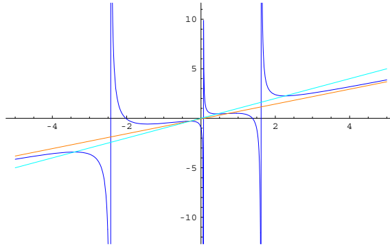
FIGURE 3. Graphics of Newton map N_{-1,8} in region \mathcal{R}_5
