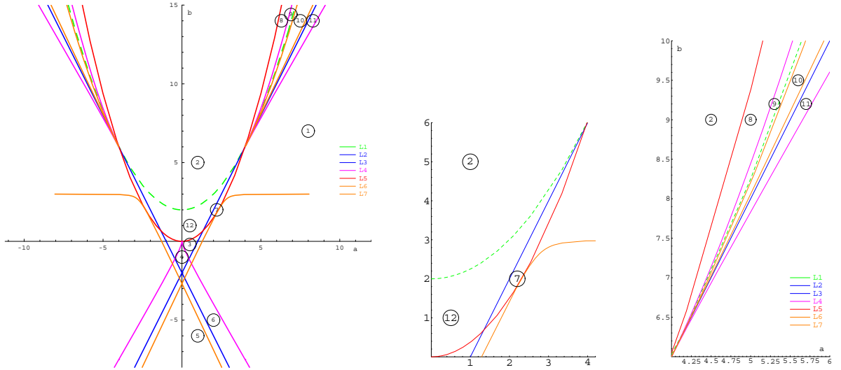
FIGURE 2. Regions in parameter plane bounded by the curves L_1, L_2, L_3, L_4 and L_5 and two zooms. The curves L_6 and L_7 , corresponding to a collision of the roots of p and p'' , are also drawn since they play an important role in the arguments.
