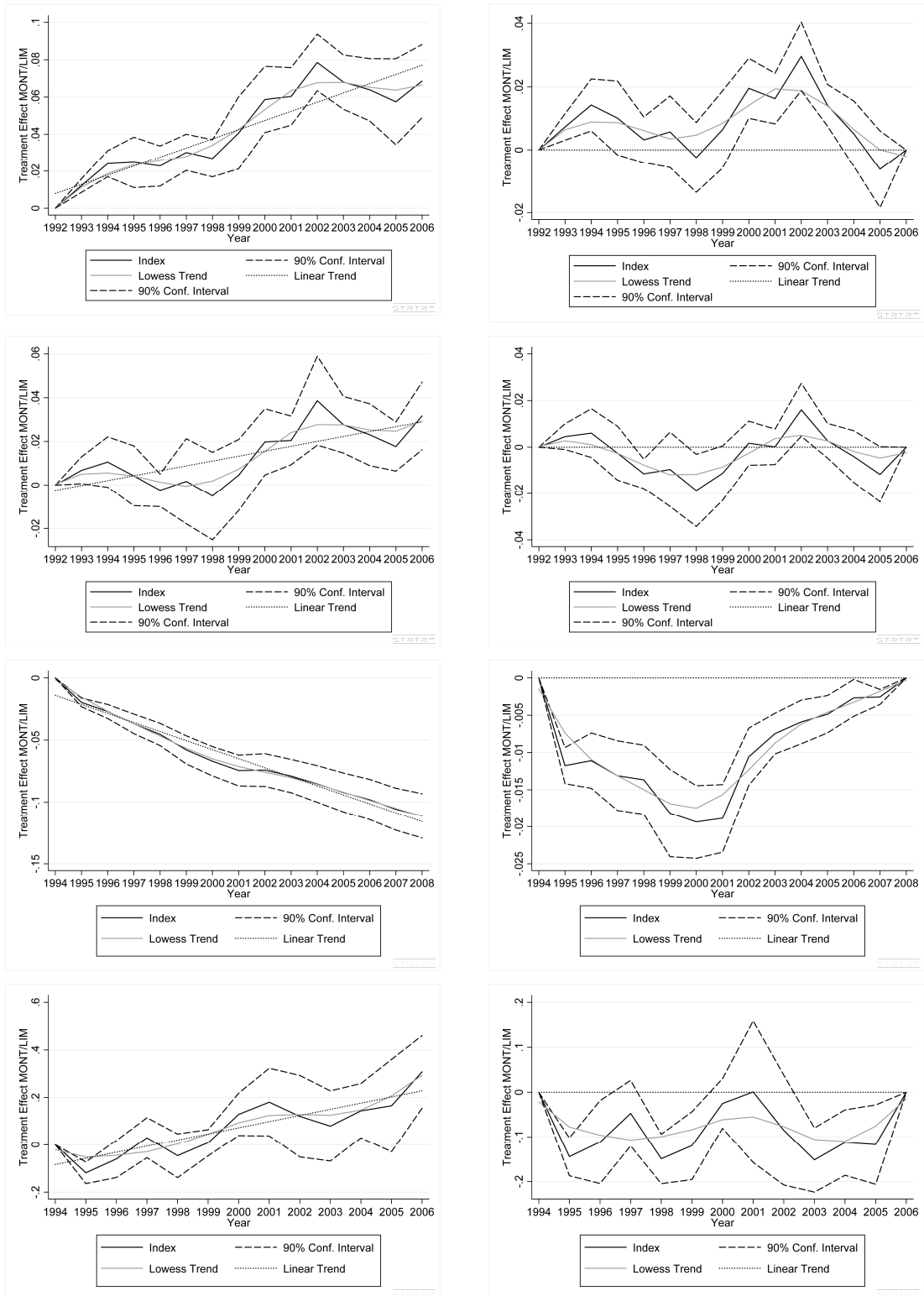
Fig. 4 Discrete Treatment ( x^b )
