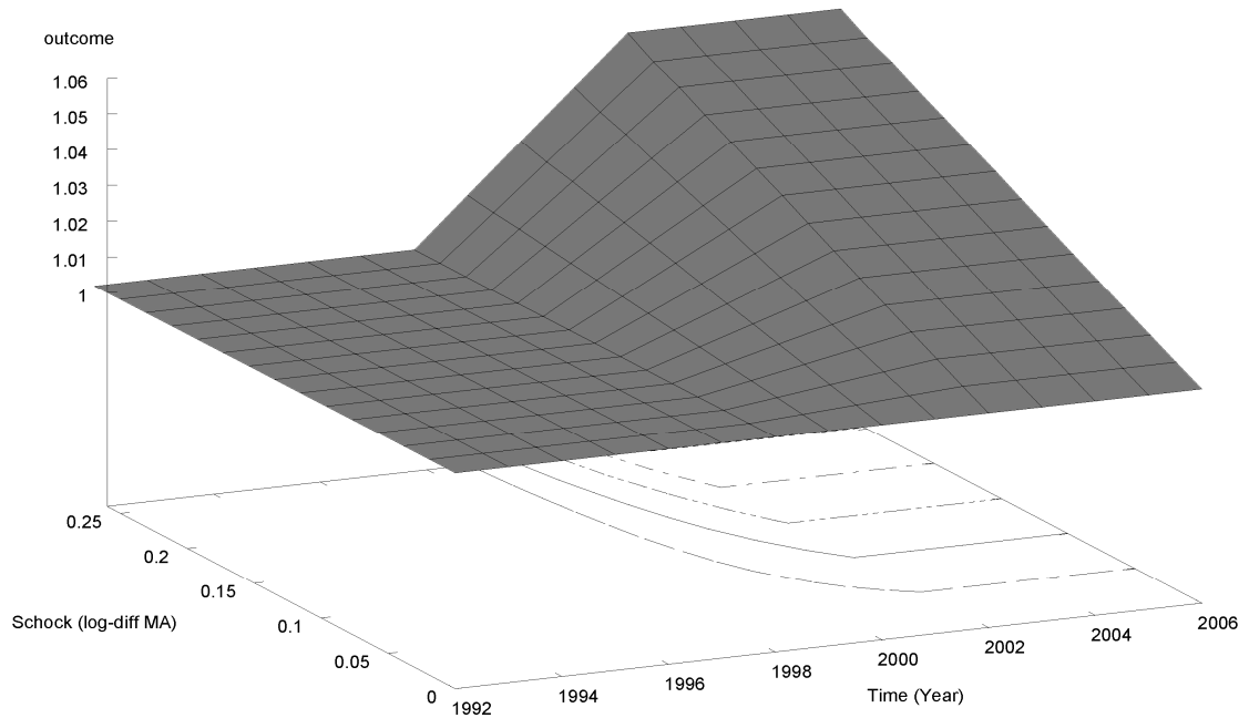
Fig. 2 Outcome variable surface
