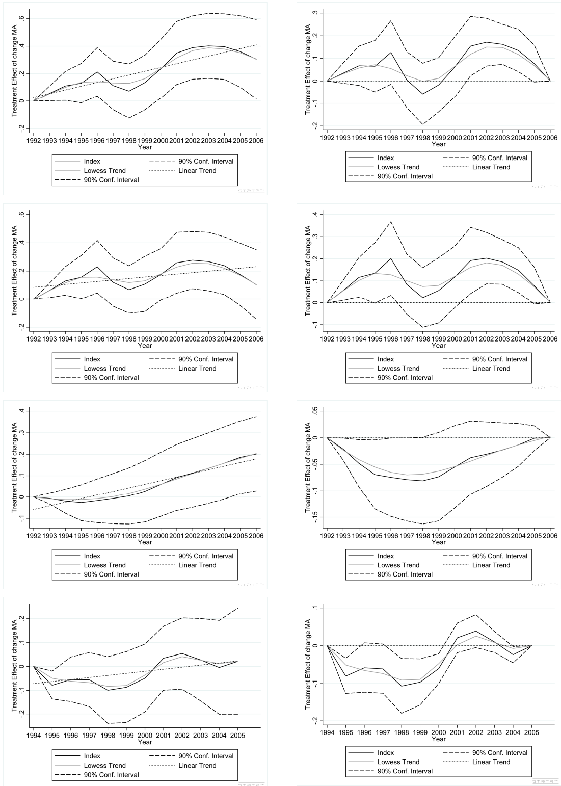
Fig. 3 Market Access Treatment ( x^a )
