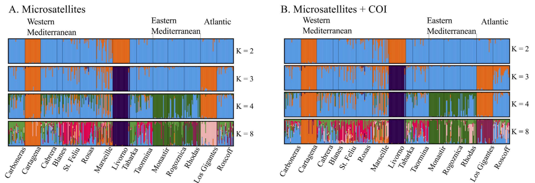
Figure 3. Bar plots of the Bayesian clustering analysis obtained using STRUCTURE for different K values. (A) Analysis based on microsatellite loci. (B) Analysis based on the combination of both mitochondrial sequences (COI) and microsatellite loci. Note that the same K values are presented, for comparison between databases.
