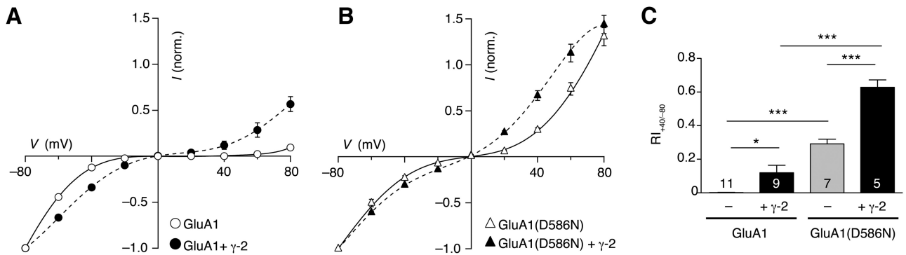
Figure 5. Neutralizing charge at the Q/R +4 position of GluA1(D586N) reduces polyamine block of CP-AMPA receptors but does not affect TARP-induced attenuation of block. A , I - V relationships for glutamate-evoked peak responses (10 mM) between -80 and +80 mV in outside-out patches from cells expressing GluA1 homomers ( n = 11 ) and GluA1 + \gamma -2 ( n = 9 ). Symbols indicate the mean and error bars (when visible) \pm SEM. B , As for A but with GluA1(D586N) homomers ( n = 7 ) and GluA1(D586N) + \gamma -2 ( n = 5 ). C , Pooled RI_{+40/-80} values for GluA1 and GluA1(D586N) homomers alone and with \gamma -2. Mean values and SEM are shown; numbers in bars denote the number of patches. Two-way ANOVA revealed a significant main effect of AMPAR mutation ( F_{(1,28)} = 135.67 , p < 0.001 ), a significant main effect of TARP ( F_{(1,28)} = 32.68 , p < 0.001 ), and a significant interaction between AMPAR and TARP ( F_{(1,28)} = 8.88 , p < 0.01 ). * p < 0.05 , *** p < 0.001 , results of pairwise comparisons (unpaired Welch two-sample t tests with Holm's sequential Bonferroni correction).
