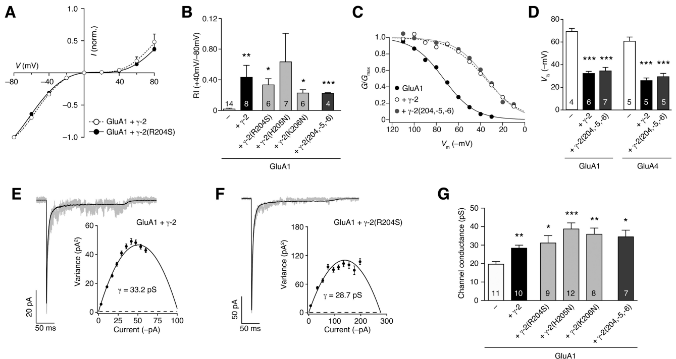
Figure 2. Mutations in the \gamma -2 C-tail do not affect polyamine block or channel conductance. A , I - V relationships for peak glutamate-evoked (10 mM) responses recorded between -80 and +80 mV in outside-out patches from cells expressing GluA1 + wild-type \gamma -2 ( n = 4 ) or GluA1 + \gamma -2(R204S) ( n = 4 ). Error bars denote SEM. B , Pooled data showing the RI (measured as the peak current at +40 mV/peak current at -80 mV) for GluA1 + \gamma -2 and mutated versions of \gamma -2. Mean values and SEM are shown; numbers in columns denote the number of patches. The RI differed across the six groups (one-way ANOVA, F_{(8,14.5)} = 6.74, p < 0.001 ). Differences between GluA1 alone and wild-type or mutant \gamma -2 are indicated (* p < 0.05 , ** p < 0.01 , *** p < 0.001 ; unpaired Welch two-sample t tests with Holm's sequential Bonferroni correction). All mutants p > 0.05 compared with wild-type \gamma -2. C , Representative normalized G - V relationships for peak glutamate-evoked (10 mM) responses recorded between -110 and -10 mV in three outside-out patches from cells expressing GluA1, GluA1 + wild-type \gamma -2, or GluA1 + \gamma -2(204, -5, -6). Lines are fits to a Boltzmann equation (Eq. 3; see Materials and Methods). For the examples shown, V_{1/2} was shifted from -73.4 mV for GluA1 to -35.7 mV for GluA1 + wild-type \gamma -2 and to -34.4 mV for GluA1 + \gamma -2(204, -5, -6). D , Pooled data showing V_{1/2} values for GluA1 and GluA4 either alone or coexpressed with \gamma -2 or \gamma -2(204, -5, -6). Columns and error bars indicate mean values and SEM; numbers in columns denote the number of patches. Two-way ANOVA showed a significant main effect for the AMPAR ( F_{(1,26)} = 9.17, p < 0.01 ), a significant main effect for TARP ( F_{(2,26)} = 90.37, p < 0.001 ), and no significant interaction ( F_{(2,26)} = 0.14, p = 0.87 ). *** p < 0.001 , differences between GluA1 alone and wild-type and mutant \gamma -2 (unpaired Welch two-sample t tests with Holm's sequential Bonferroni correction). E , Currents elicited by rapid application of 10 mM glutamate (200 ms) to an outside-out patch from a tsA201 cell ( -60 mV) transfected with GluA1 + \gamma -2. A single raw trace (gray) is shown overlaid with the mean response (black). The inset shows the current-variance plot for the same recording. The fitted parabola (see Materials and Methods) gave a weighted single-channel conductance of 33.2 pS. Dashed line denotes background variance, and error bars denote SEM. F , Same as in E but for a patch from a cell expressing GluA1 + \gamma -2(R204S); the fitted parabola gave a weighted mean single-channel conductance of 28.7 pS. G , Pooled weighted mean single-channel conductance data from NSFA of GluA1 + wild-type and mutated versions of \gamma -2. Mean values and SEM are shown; numbers in bars denote the number of patches. Weighted mean conductance differed significantly across the six groups (one-way ANOVA, F_{(8,26.7)} = 5.96, p < 0.001 ). Multiple pairwise comparisons (unpaired Welch two-sample t tests with Holm's sequential Bonferroni correction) revealed differences between GluA1 alone and GluA1 expressed with wild-type or mutant \gamma -2 (* p < 0.05 , ** p < 0.01 , *** p < 0.001 ). All mutants p > 0.05 compared with wild-type \gamma -2.
