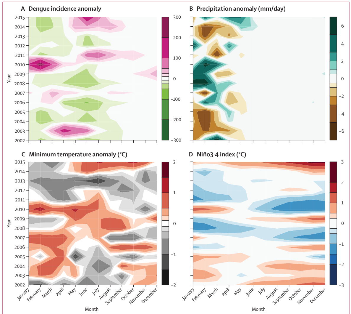
Figure 1: Annual cycle of anomalies in dengue and climate variables, 2002-15 (A) Dengue incidence anomalies in Machala, Ecuador per 100 000 population. (B) Precipitation anomalies (mm/day). (C) Minimum temperature anomalies (°C), from the Granja Santa Ines weather station, located in Machala. (D) Niño3-4 index (sea surface temperature anomalies [°C] in the Niño3-4 region).
