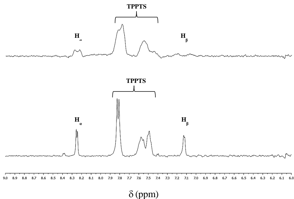
Figure 1. ^1\text{H-NMR} spectrum of 1 at 1 \cdot 10^{-3}\text{M} (up) and 1 \cdot 10^{-4}\text{M} (bottom) concentrations in \text{D}_2\text{O} .
