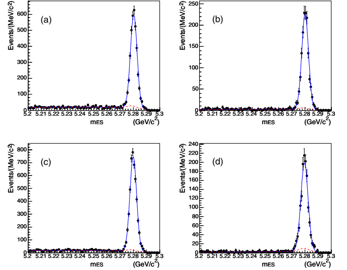
FIG. 1 (color online). Fit of m_{\text{ES}} distributions for the B \rightarrow D^{(*)}\pi candidates in data: (a) \bar{B}^0 \rightarrow D^+\pi^- , (b) \bar{B}^0 \rightarrow D^{*+}\pi^- , (c) B^- \rightarrow D^0\pi^- , (d) B^- \rightarrow D^{*0}\pi^- . The fit is shown as a solid line and is described in the text. The background component (including peaking background) is shown as a dashed line.
