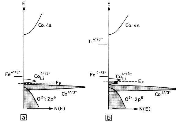
FIG. 4. Schematic energy diagrams illustrating the Auger-electron capture process at \text{Co}^{4+} associated with a native defect ( \text{Li}^+ -ion vacancy) in a (a) p -type sample, and (b) Ti-doped sample.
