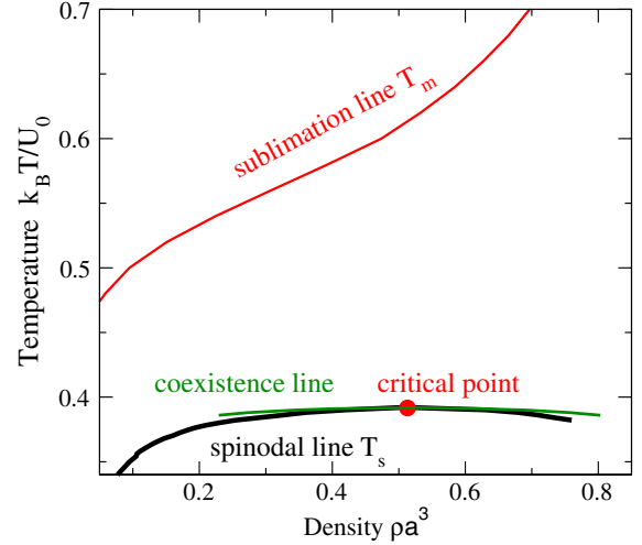
FIG. 1 (color online). T - \rho phase diagram for the potential in Eq. (3). Below the sublimation line, we calculate the metastable gas-liquid spinodal line by connecting minima and maxima along the isotherms in the P - \rho plane and the coexistence line from the equal-area Maxwell construction in the P - V plane. The point of merging of these two lines corresponds to the metastable critical point. By interpolating the minima of the inverse compressibility for the isotherms at T = 0.392U_0/k_B and T = 0.391U_0/k_B , we locate the critical point at T_c = (0.3916 \pm 0.0005)U_0/k_B , \rho_c = (0.523 \pm 0.005)(1/a^3) , and P_c = (0.0519 \pm 0.0005)U_0/a^3 , with T_c/T_m \approx 0.64 at \rho_c .
