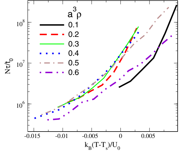
FIG. 3 (color online). The scaling of the crystal nucleation time \tau with respect to the spinodal temperature T_s , proposed by Vaiana et al. , only holds for the subcritical range 0.2 < a^3 \rho < 0.5 but fails outside of it. Lines correspond to different densities.
