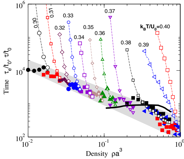
FIG. 2 (color online). Equilibration time \tau_e (closed symbols) and nucleation time \tau (open symbols) as function of density \rho for different temperatures T (labels near symbols) in units of U_0/k_B . At each \rho , the metastable fluid is defined only when \tau > \tau_e , above the gray area; otherwise, the crystallization is instantaneous compared to \tau_e . Along the spinodal line, the values of \tau (connected by a solid line) are larger than \tau_e only for 0.38 \leq k_B T/U_0 \leq 0.39 and \rho > 0.3/a^3 .
