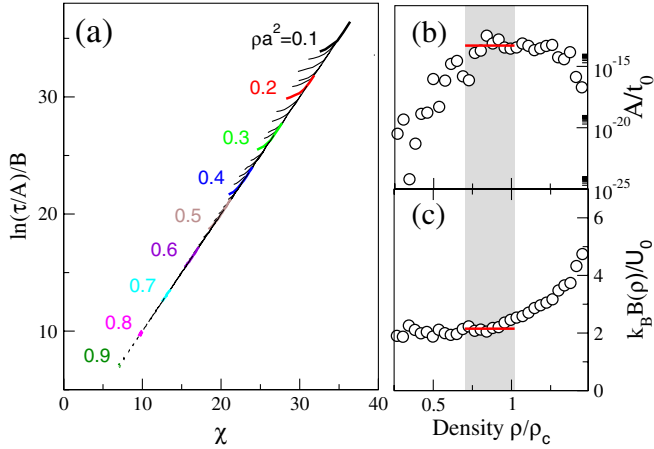
FIG. 5 (color online). (a) Scaling plot of nucleation time \tau along different isochores (with labels near lines for a selected number of them) following Eq. (2) with strongly \rho -dependent A and B parameters. Deviations from the straight line occurs for \tau \approx \tau_e (gray region in Fig. 2). (b) The \rho dependence of A , inverse of the kinetic prefactor \kappa , as resulting from our fitting to collapse data in (a). The shaded region corresponds to the density range of the critical iso-CNT line, where A \approx 5 \times 10^{-14} t_0 (horizontal line). Around the critical density, A reaches a maximum plateau and \kappa is minimum. (c) The \rho dependence of B , in units of U_0/k_B , from the fitting in (a). B increases approaching \rho_c from subcritical densities. The red line (at B = 2.15 U_0/k_B ) is a guide for the eyes, the shaded region is as in (b).
