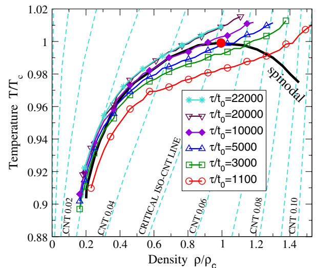
FIG. 4 (color online). The loci of equal \tau (symbols) are compared with the iso-CNT lines (dashed lines) for different values of CNT parameter \chi (labels near dashed lines, expressed in units of U_0/k_B ) and the spinodal (solid) line, the vertex of which is the metastable critical point (full circle).
