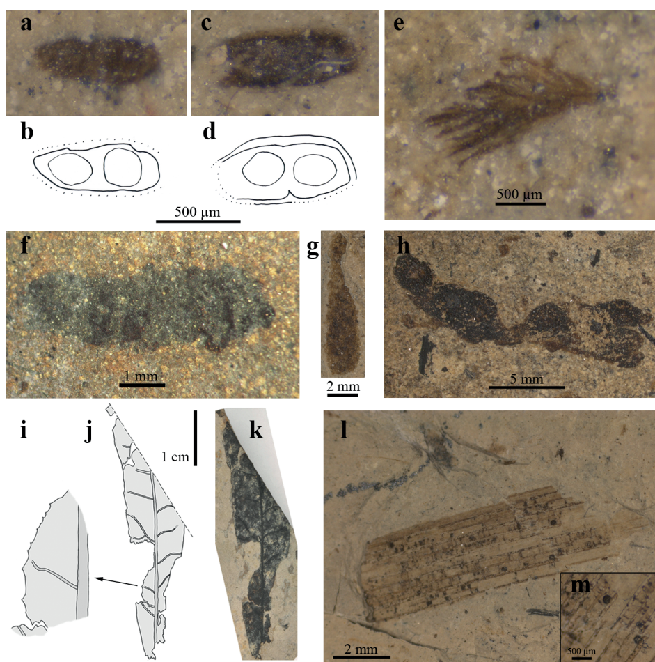
Figure 4. Photographs and drawings of San Chils fossils. a-d) Daphnia ( Ctenodaphnia ) sp. ephippia; ( a-b ), SC-114A, ( c-d ), SC-115A. e) Bird feather indet., SC-99A. f-h) Coprolites; ( f ), SC-28, ( g ), SC-101B, ( h ), SC-116. i-k) Myrica sp. leaf with margin feeding, SC-7. l-m) Monocotyledon leaf with possible piercing/sucking marks, SC-110. Each pair of photograph and drawing in a-b, c-d and j-k is at the same scale.
