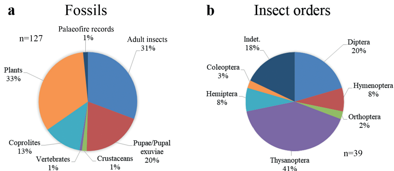
Figure 6. a) Representation of the percentage of types of fossils recorded in San Chils. b) Representation of the percentage of insect orders in San Chils fossil record.
