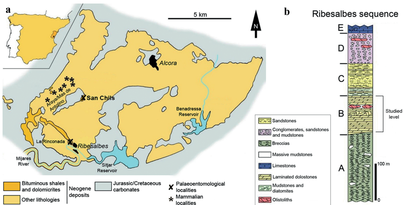
Figure 1. a) Geological map of the Ribesalbes-Alcora Basin showing the known palaeontomological and the mammalian localities. Modified from Peñalver et al. (2016). b) Stratigraphic column of the Ribesalbes sequence with the indication of the units A to E. Modified from Anadón et al. (1989), Barrón & Postigo-Mijarra (2011) and Crespo et al. (2019).
