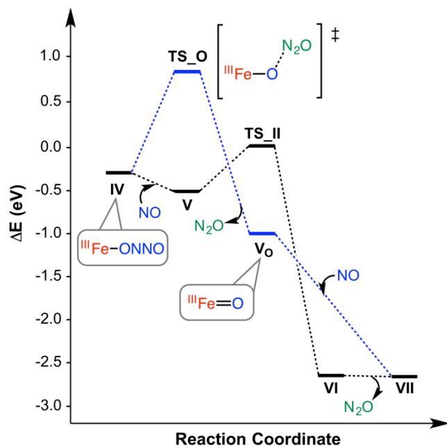
Scheme 4. Proposed reaction pathways from intermediate IV . Black line = pathway in Scheme 2; blue line = formation of iron-oxo intermediate (energies in eV).
