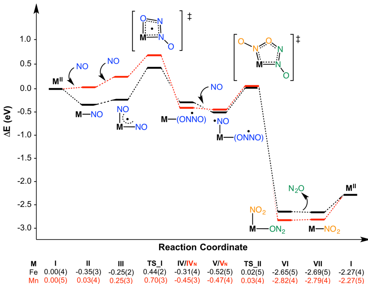
Scheme 5. Relative energy profiles for the Fe- and Mn-MOF-5 catalyzed NO disproportionation (M: Fe = black, Mn = red, energies in eV, unpaired electrons are given between brackets).
