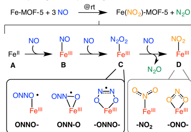
Scheme 1. NO disproportionation reaction, including the proposed mechanism and plausible species in the Fe-MOF-5 catalyzed NO disproportionation. Adapted with permission from J. Am. Chem. Soc. 2015 , 137 , 7495-7501. Copyright (2015) American Chemical Society.
