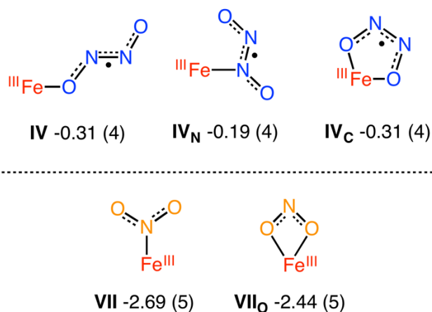
Scheme 3. Possible isomeric species of compounds IV (top) and VII (bottom): energies are given in eV and the number of unpaired electrons of each species is given between brackets.
