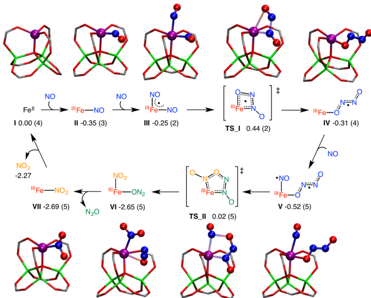
Scheme 2. Computed reaction pathway for the Fe-MOF-5 catalyzed NO disproportionation. Energies are given in eV, the number of unpaired electrons of each species is given between parentheses. Color code of the Fe core: C = gray, N = blue, O = red, Fe = purple, Zn = green; atoms represented as balls correspond to those actively participating in the reaction steps.
