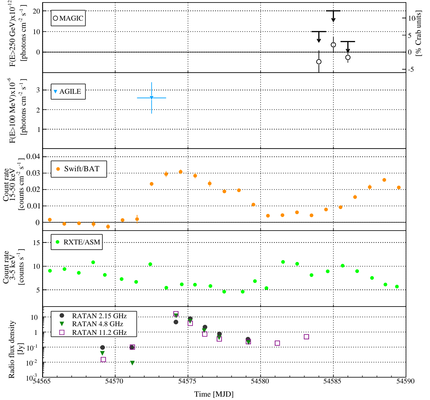
FIG. 8.— Zoom of Figure 2 around the cycle IV campaign between 2008 April 9 and May 2. The open black points in the VHE MAGIC panel show the non-significant measured integral fluxes with their statistical error bars (whereas the ULs take into account also the systematic errors).
