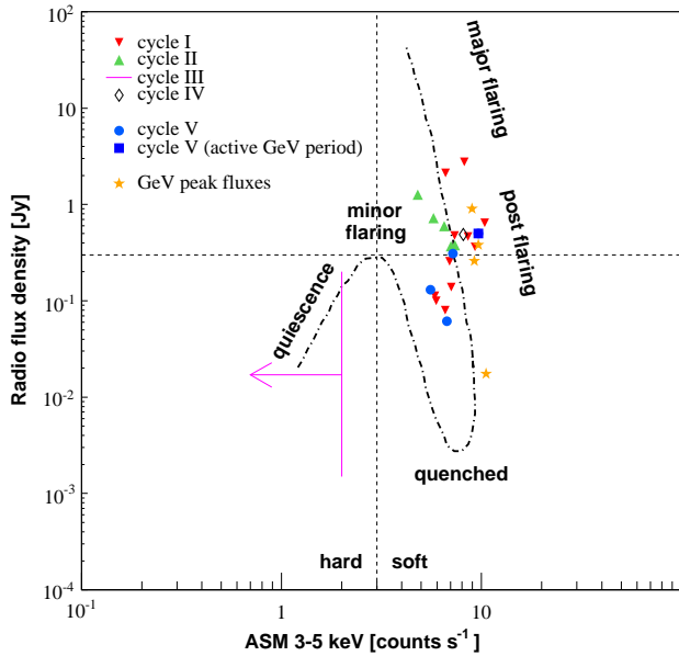
FIG. 7.— Soft X-ray counts vs. radio fluxes simultaneous with the GeV peak fluxes (yellow stars) and MAGIC observations, where the different marker colors identify the five MAGIC observational cycles. The pink arrow shows the X-ray flux level during the cycle III MAGIC campaign, for which radio data are not available. Radio measurements are at 11.2 GHz from RATAN-600 and at 15 GHz from RT/AMI. The dot-dashed line shows the expected “saxophone” shape, adapted from Szostek et al. (2008).
