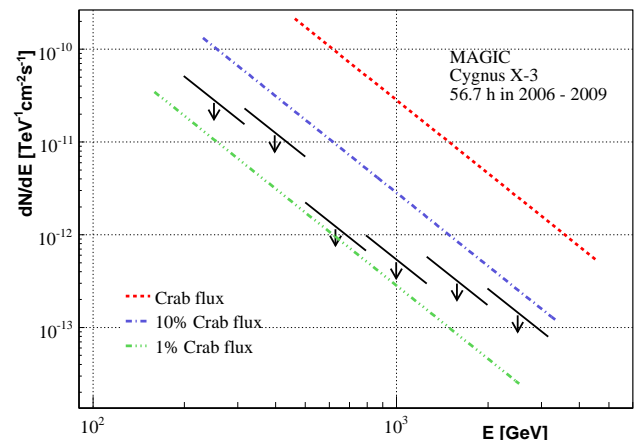
FIG. 1.— Differential flux ULs at 95% CL for the VHE time-integrated emission. The slope of the arrows indicates the assumed power-law spectrum with a photon index of 2.6.
