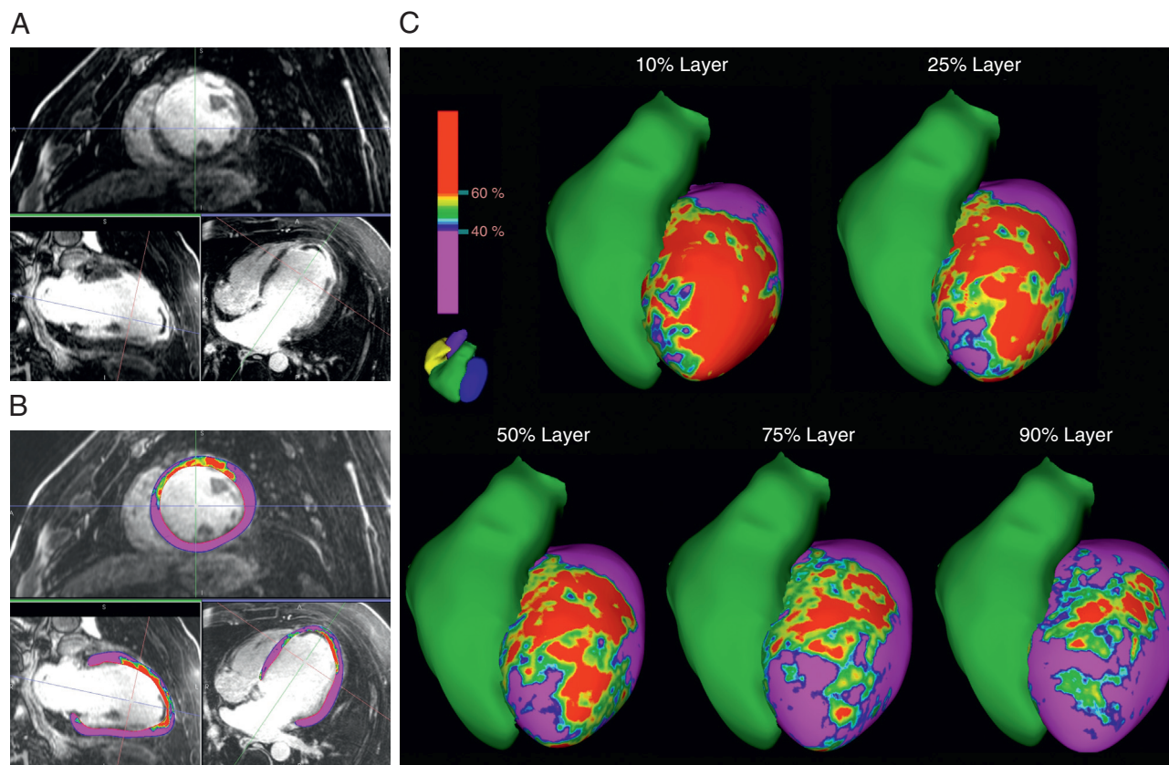
FIGURE 1 Image Processing
