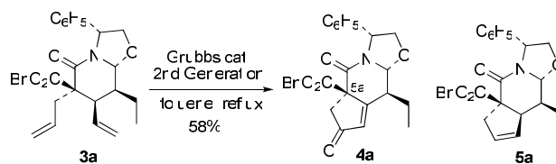
Scheme 2. Unexpected Oxidation in the Cyclopenta[ c ]piperidine Series
