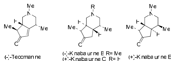
Figure 1. Alkaloids with a 6-oxocyclopenta[ c ]piperidine skeleton.
