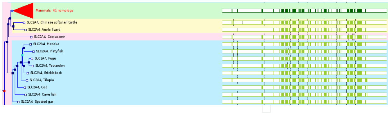
Figure 1. Evolutionary tree of the GLUT4 gene (SLC2A4) in vertebrates. Alignment of the different GLUT4 gene sequences is shown on the right. White sections of the alignment indicate gaps in the sequence.
