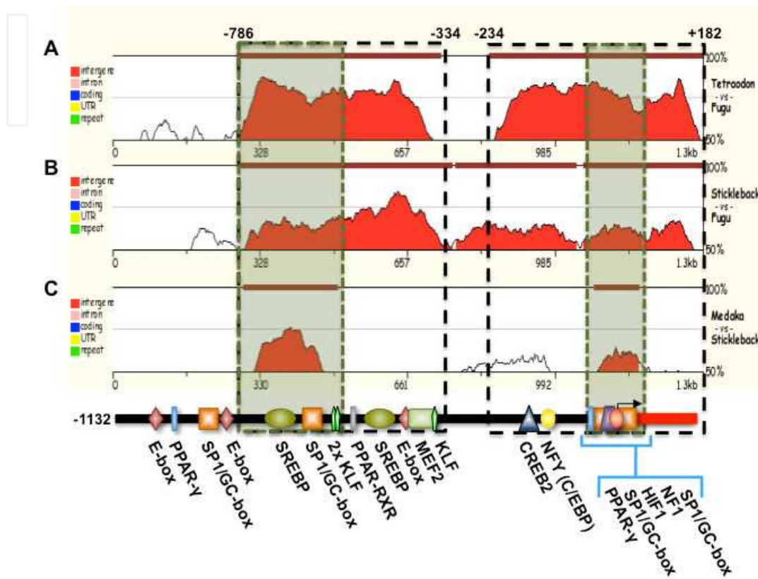
Figure 4. Conservation profile of the promoter region of known fish GLUT4 genes. Sequence elements of significant length ( \geq 100 nucleotides) that show higher than 60% of homology are highlighted in red and depicted with the dark-red rectangles on the top of each graph. The sequence comparison between the Fugu and Tetraodon (A), Fugu and Stickleback (B) and Stickleback and Medaka (C) GLUT4 promoters is shown. The horizontal axis represents the position of the nucleotides within the 1314 bp sequence compared, starting at the 5' end. The vertical axis represents the percent of identity between the aligned genomes. In the bottom, a schematic representation of the -1132 Fugu GLUT4 gene promoter highlighting the most relevant predicted binding sites is shown. The open boxes delineating the regions comprised between -786/-334 and -234/+182 nucleotides represent conserved areas in fish GLUT4 gene promoters. Adapted from [30].
