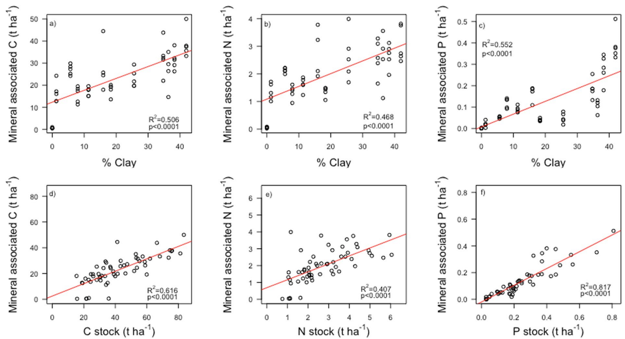
Figure 3. Mineral associated carbon (C) Nitrogen (N), phosphorus (P), and isolated by density and size fractionation and their association with, (a–c) clay (<2 μm) content of the soil, and (d–f) total elemental stocks in the top 15 cm of the soil. Stocks were calculated by multiplying elemental concentrations by bulk density.
