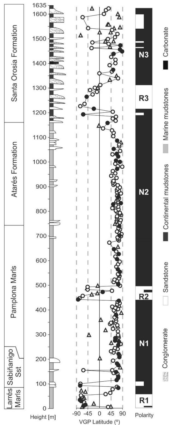
Figure 4.8: Yebra de Basa (Jaca Basin) magnetostratigraphic section. Black dots represent high-quality paleomagnetic directions and white dots represent intermediate quality. Triangles represent low-quality paleomagnetic directions.
