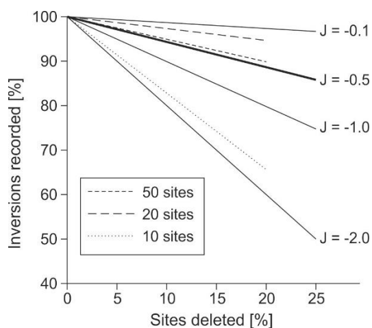
Figure 3.10: Example of a Jackknife test after different simulations, redrawn from Tauxe and Gallet (1991). Observe that as more sites are collected in a section, less slope (J) has the linear regression. It is estimated that a magnetostratigraphic section has captured the significant chrons if J is higher than -0.5.
