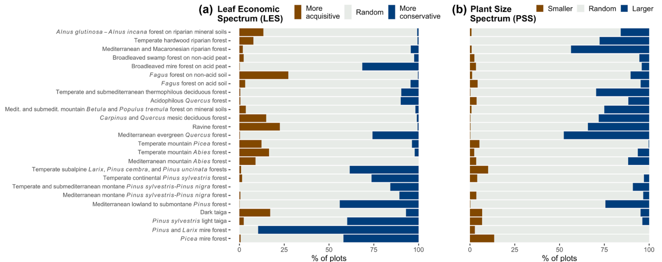
Figure 5. Proportion of plots from forest types with understories containing plant species with (a) more acquisitive (brown) and conservative (blue) leaf economics than under random expectation, and with (b) smaller (brown) and larger (blue) plant and seed sizes than under random expectation, based on CWM.ses of the leaf economic spectrum (LES) and plant size spectrum (PSS), respectively. The proportion of plots with random LES and PSS are shown in light grey.
