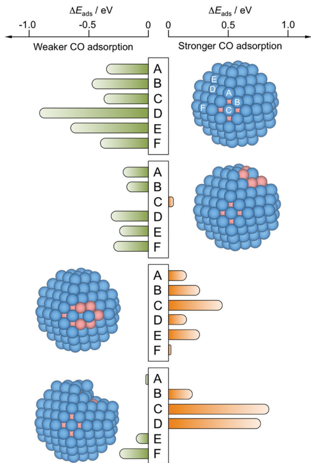
Fig. 5 Differences in CO adsorption energies, \Delta E_{\text{ads}} , on PtCu NPs with respect to reference Pt 201 NP, calculated for all topologically different top sites, see Fig. S1 of the ESI.† From top to bottom, perfect Cu@Pt core@shell NP— model 3 , see Fig. 4—with a surface Pt atom fully coordinated to Cu atoms— model 6 —, with a surface Pt atom coordinated to surface Cu atoms— model 7 —, and model 8 resulting from removal of five surface Cu atoms from model 7 and subsequent optimization. Sites A–D are shown in model 1 but are the same for the rest of models 6–8 .
