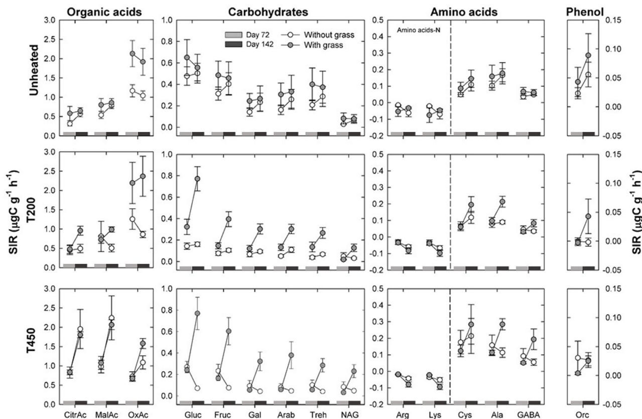
FIGURE 3 Substrate-induced respiration (SIR) (mean \pm standard error, n = 5 ) of unheated and heated soils. For each heating and grass treatment, couples of SIR values for each substrate provide mean SIR ( n = 5 ) at days 72 (left circles) and 142 (right circles) of the incubation. Given the observed different behaviour of arginine and lysine (i.e., those richest in N) from the other amino acids, they were analysed separately, as indicated by the vertical dashed line. Note the change in scale between types of substrate
