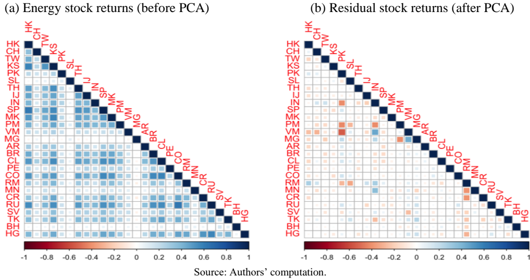
Figure 2. Unconditional correlation matrix for energy stock returns at country level
