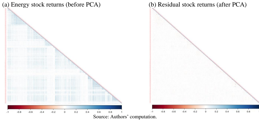
Figure 3. Unconditional correlation matrix for energy stock returns at firm level
