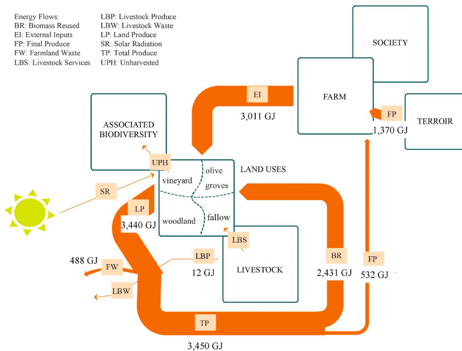
Fig. 3. Sankey flowchart of the main energy flows and returns of the Gramona farm system.
