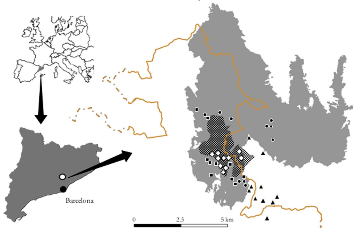
Fig. 1 Location of study area and distribution of sampling plots. Location of the Sant Llorenç del Munt i l'Obac Natural Park, with its border (orange line) in Catalonia (NE Iberian Peninsula), the 2003-burnt shape and size (grey), the historical (1970 and 1994) burnt areas (grated), and the forty 100×100 m plots, where black trian-
