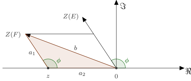
FIGURE 2. The left-hand side of \text{HN}_{\mathcal{A}}^Z(F) is contained in the triangle 0, z, Z(F) .
