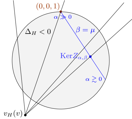
FIGURE 1. Walls in the cross-section of the negative cone
