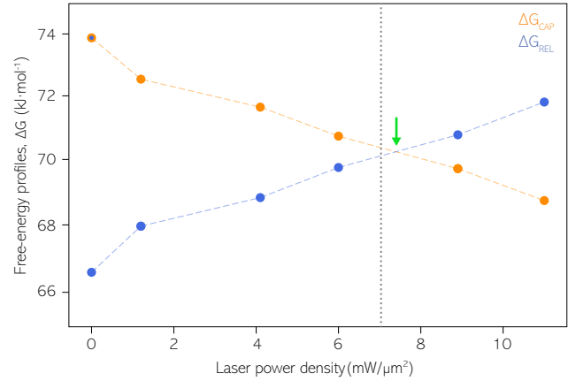
Fig. 5 Capture and release barriers, \Delta G_{REL} and \Delta G_{CAP} , respectively, as a function of the laser power density. The dashed lines are a guide to the eye. Vertical dashed line at 7.1 mW/\mu m^2 indicates the transition where K_{ASS} becomes larger than K_{DIS} according to Figure 4. Green arrow indicates the intersection point between \Delta G_{REL} and \Delta G_{CAP} trends.
