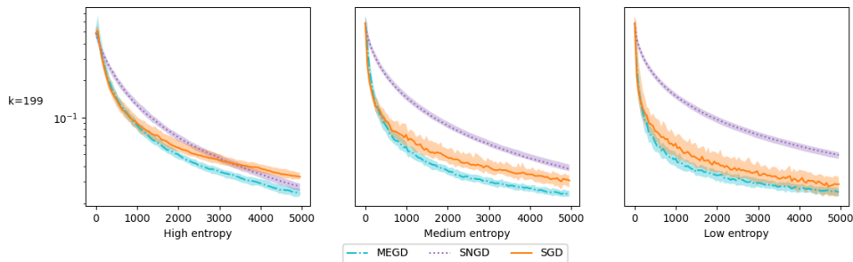
Figure 3.2: KL-Divergence of estimations per iteration of SGD , SNGD and MEGD on the die problem.
