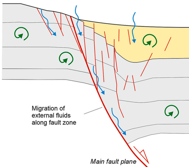
Fig. 1. Schemes showing the relationships between the evolution of fault zones in carbonate rocks and fluid flow. The extensional system is based on Baqués et al. (2010) and the compressional system on Muñoz-López et al. (2020a).
