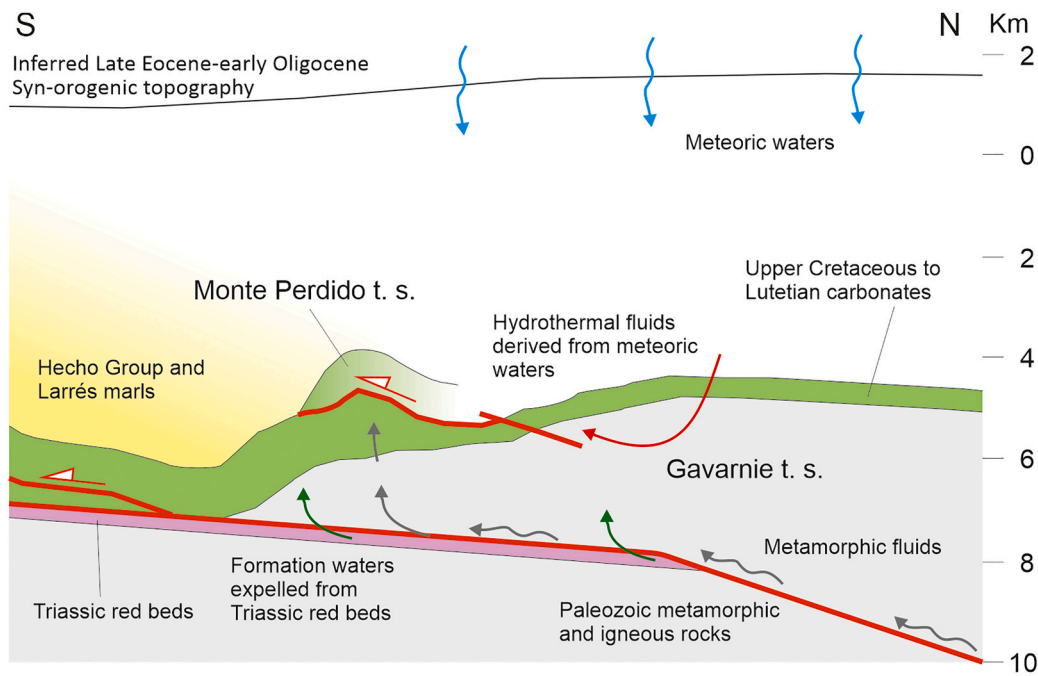
Fig. 7. Fluid flow model of the Pyrenean Axial Zone based on McCaig (1988) , Grant et al. (1990) , Banks et al. (1991) , McCaig et al. (1990, 1995, 2000) , Losh (1989) , Trincal et al. (2017) , Muñoz-López et al. (2020b) and Bradbury and Woodwell (1987) using the Gavarnie thrust sheet as an example. The cross-section is based on the restoration of Labaume et al. (2016) during the late Eocene-early Oligocene. In this model, metamorphic fluids derived from the basement and formation waters trapped in Triassic rock pores migrate into cover thrust sheets (in green). Also, meteoric waters percolate and are heated at depth, evolving into hydrothermal fluids. (For interpretation of the references to colour in this figure legend, the reader is referred to the web version of this article.)
