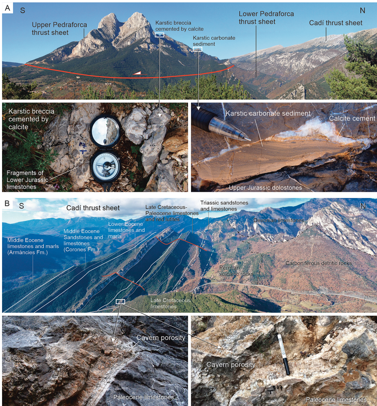
Fig. 10. Field images showing diagenetic patterns related to meteoric water migration in the southern Pyrenees. A) Meteoric calcite cement together with karstic sediments and between breccia clasts in Jurassic dolostones and limestones of the Upper Pedraforca thrust sheet. The fluids from which these cements precipitated were studied by Cruset et al., 2021, 32 in Fig. 2). B) Cavern porosity in Paleocene limestones filled by meteoric calcite at the northern sector of the Cadí thrust sheet.
