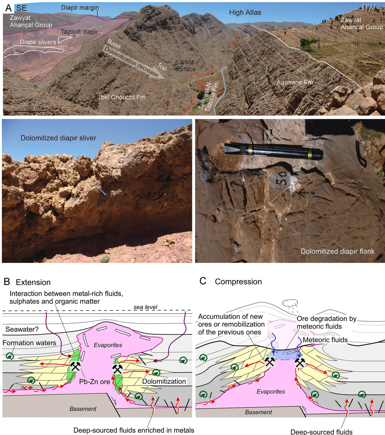
Fig. 15. A) Field images of replacive dolomite related to salt-related extension in the Tazoult Diapir, High Atlas (large-view image redrawn from Martín-Martín et al., 2017). Replacement by dolomite occurred both in carbonate slivers within the diapir core and their flanks. Photographs courtesy of Vinyet Baqués. B–C schematic cross-sections modified from Moragas et al. (2020) showing the fluid-rock interactions in diapirs in both extensional B) and compressional C) tectonic settings.
