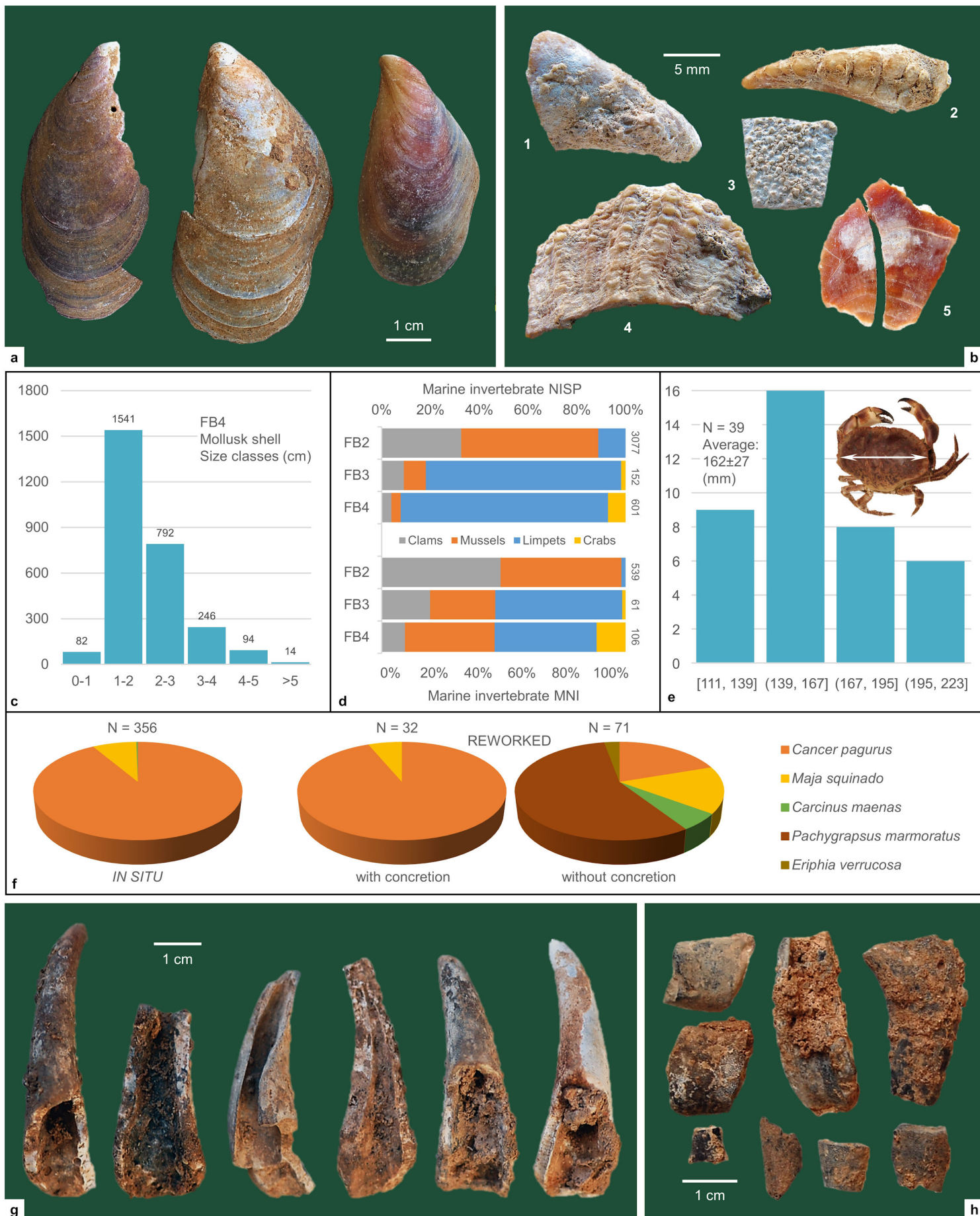
Fig. S24. Marine invertebrate taphonomy. a. Intrusive mussel shells in the small mammal burrow of T9SW (unit IT0). b. Crab claw (1-2), crab carapace (3), limpet (4) and mussel (5) shell fragments sorted from wet-sieved in situ deposit (unit IH8). c. Mollusk shell breakage in the IH complex (units IH2-IH8), Phase FB4. d. Chronological variation in the frequency of the main marine invertebrates across human occupation phases. e. Histogram of brown crab carapace width (mm; in situ units only). f. Taxonomic composition (by NISP) of the in situ and reworked crab assemblages. g. Brown crab pincers with anthropogenic breaks; h. Brown crab carapace and pincer fragments, burnt.
