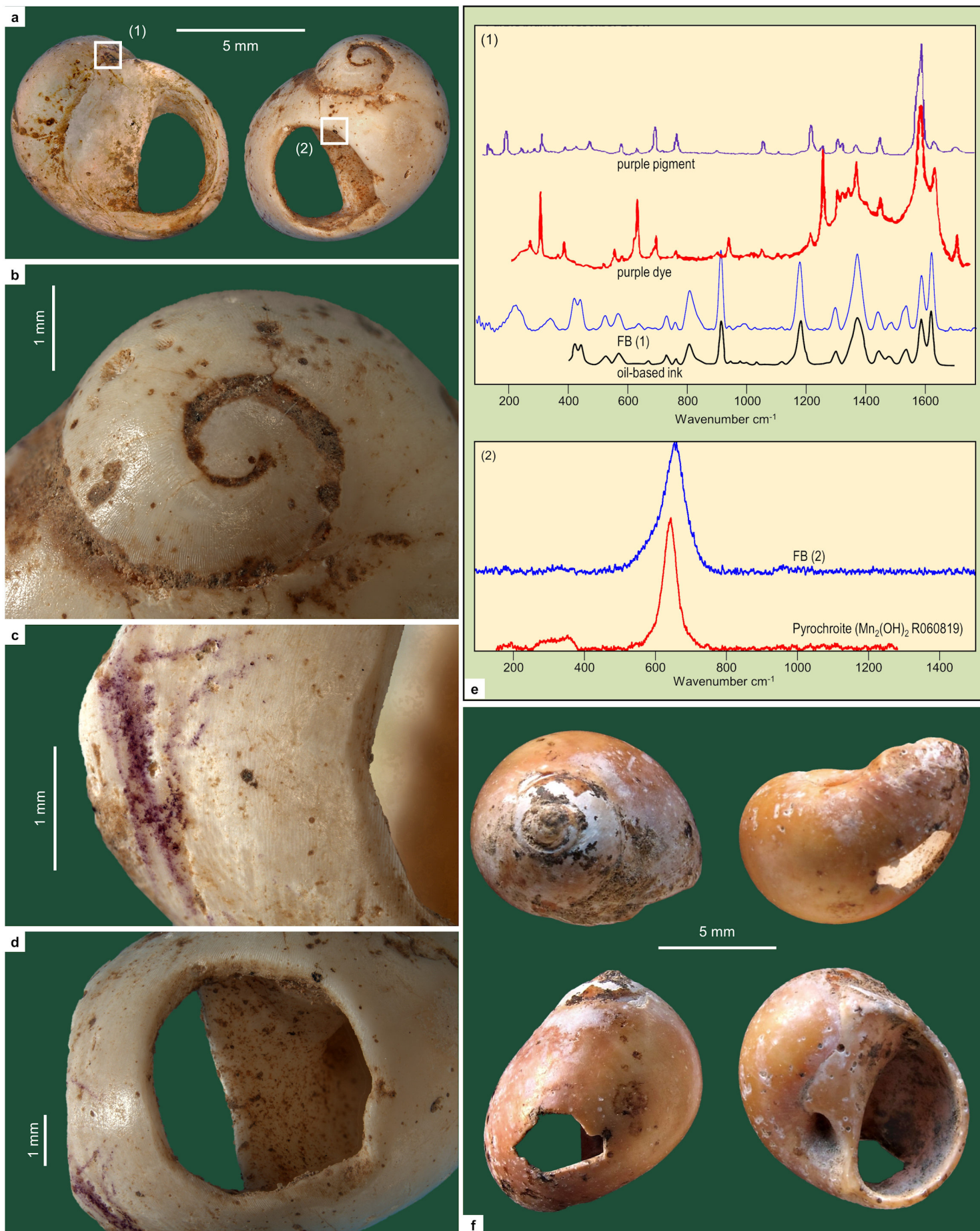
Fig. S28. The perforated gastropod shells. a. Littorina obtusata from the small mammal nest in T9-SW, reworked unit IT0, directly radiocarbon-dated to 7390 \pm 25 BP (OS-114170); the location of the two accretions analyzed by micro-Raman spectroscopy is indicated. b-d. close-up views of the L. obtusata shell; note the pitting of the surface and the well-rounded edges of the perforation. e. micro-Raman spectra (arbitrary units) of the purple (1) and black (2) accretions, which match, respectively, to a manganese mineral and an oil-based ink. f. Euspira guilleminii in the floatation sample from T9-East, unit IT2.
