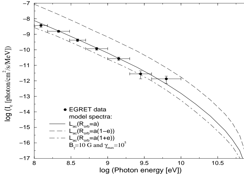
Fig. 2 Computed spectral photon distribution above 100 MeV for LS I +61 303 plotted with the EGRET data points. We have used the physical parameter values presented in Table 1. Unlike in Fig. 1, the spectral shape and the variability are the same for both B_\gamma=1 and 10 G. Thus there is only one plot. There are plotted the computed I'_e for different orbital radii: a (solid line), the distance at the periastron passage ( a(1 - e) , dashed line), and the distance at the apastron passage ( a(1 + e) , dotted line). Now, accretion changes due to orbital eccentricity have been included in calculations.
