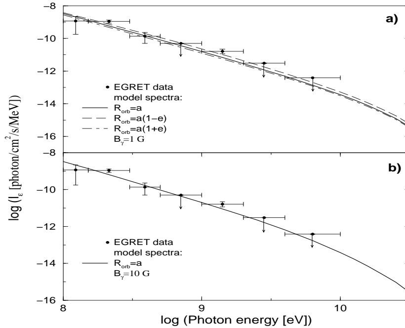
Fig. 1 Computed IC spectral photon distribution above 100 MeV for LS 5039 using the physical parameter values presented in Table 1. The EGRET data points are also shown. The upper limits on undetected EGRET points are plotted with arrows. Only stellar radiation density changes due to the orbital eccentricity have been taken into account. a) A magnetic field of 1 G has been adopted. Also, the IC spectral photon distribution for both the apastron and the periastron passage are shown. b) A magnetic field of 10 G has been adopted.
