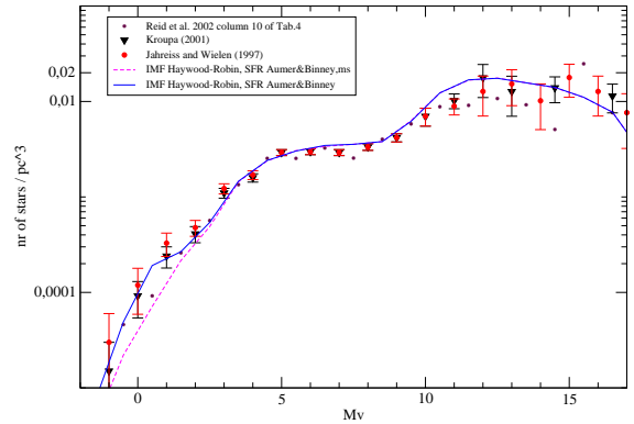
Fig. 9: Comparison of the observed LF with simulated one from model A: total LF (blue solid line) and main sequence LF (magenta dashed line). Symbols for observed data are same as in fig. 8.
