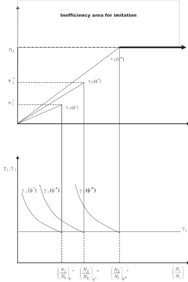
Transitional dynamics
