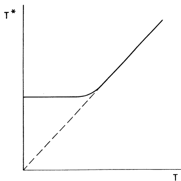
FIG. 1. Dependence T^*(T) .
