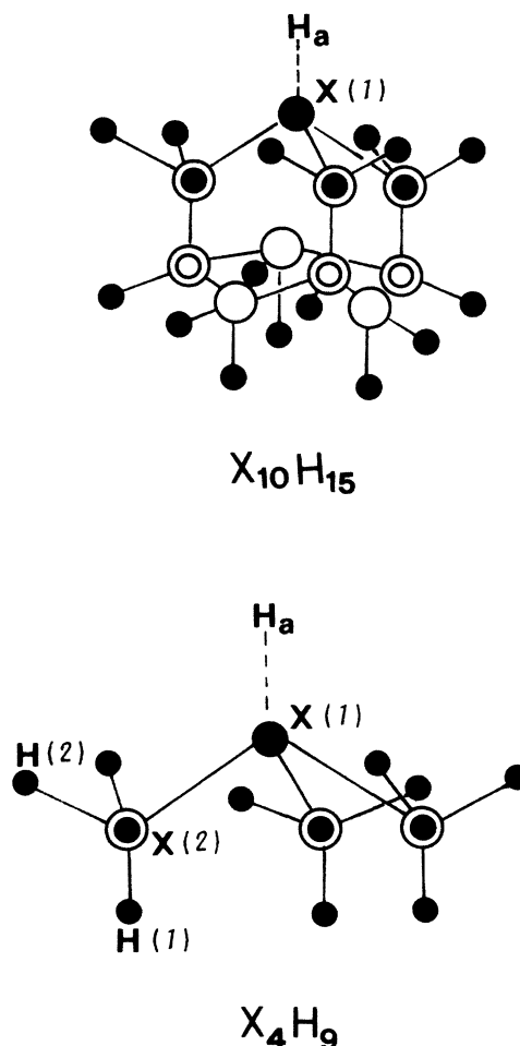
FIG. 1. Schematic drawing of the model clusters H-X_4H_9 and H-X_{10}H_{15} used in the study of hydrogen chemisorption on the (111) surfaces of diamondlike crystals.
