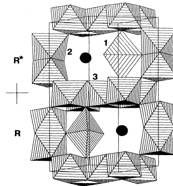
FIG. 1. STRUPLO drawing of the crystal structure of \text{BaFe}_{4-2x}\text{Sn}_{2+x}\text{Co}_x\text{O}_{11} indicating the 4f(\frac{1}{2}) , 4e , and 6g sites (labeled 1, 2, and 3, respectively) and the Ba atom sites (black circles).
