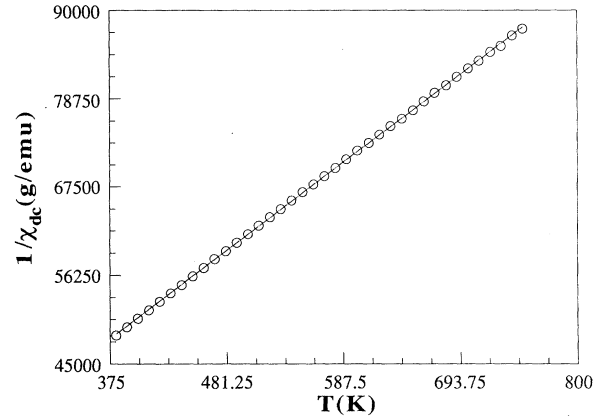
FIG. 8. Reciprocal of the dc susceptibility for the sample having x \approx 1.2 in the high-temperature range. The line represents a fit to the Curie-Weiss law.
