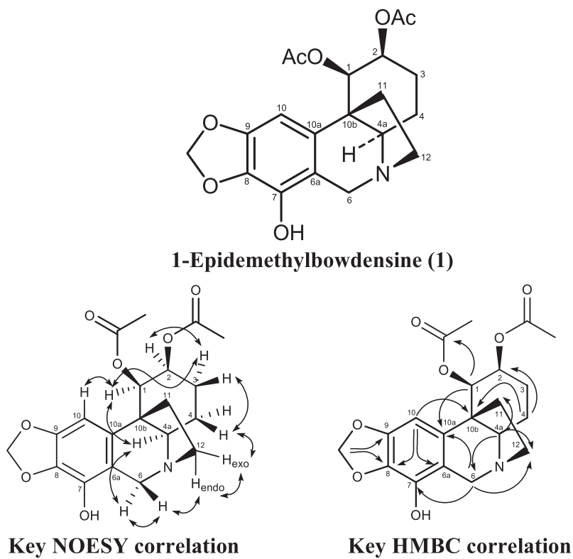
Figure 3 Key NOESY ( \leftrightarrow ) and HMBC ( \rightarrow ) correlation of compound 1.
