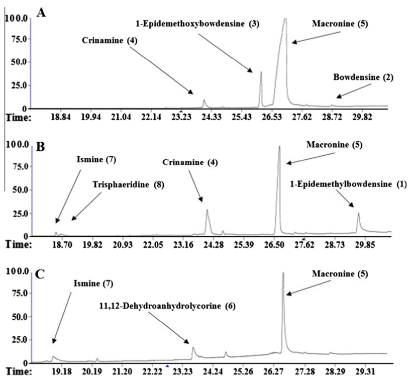
Figure 2 GC-MS chromatogram of n -Hex (A), EtOAc (B) and EtOAc:MeOH (C) extracts from Crinum erubescens with the identified alkaloids.
