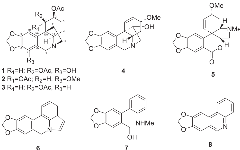
Figure 1 Alkaloids identified from Crinum erubescens .
