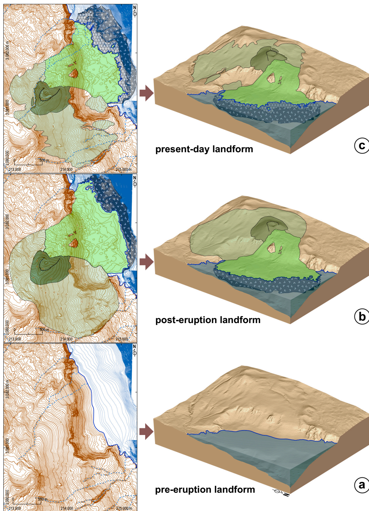
Fig. 14. Shoreline evolution of El Hierro Island's littoral affected by the Montaña del Tesoro eruption. Shoreline configuration at a generic time-frame in the present sea-level highstand (a) where the Montaña del Tesoro eruption occurs (dated at 1050 years BP) (b). A more efficient marine than fluvial erosion leads to the current scenario (c). Same legend as Fig. 10.
