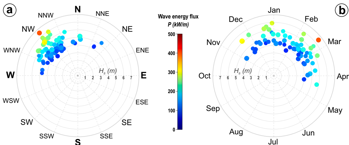
Fig. 8. Wave energy flux associated to annual maximum storms at selected computational node offshore Montaña del Tesoro, for the period 01/1958–03/2022, in terms of approach direction (a) and time of occurrence throughout the year (b).
