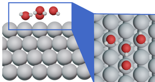
Figure 1. Side (left) and top (right) views of a cluster of four water molecules. The central water molecule is solvated by the three peripheral ones in the first solvation shell. See more configurations in Figure S2.
