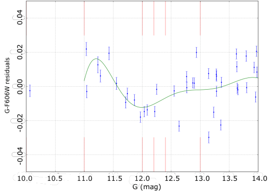
Fig. 44. Same as in Fig. 43, but for M4 using G minus HST F606W photometry by Nascimbeni et al. (2014).
