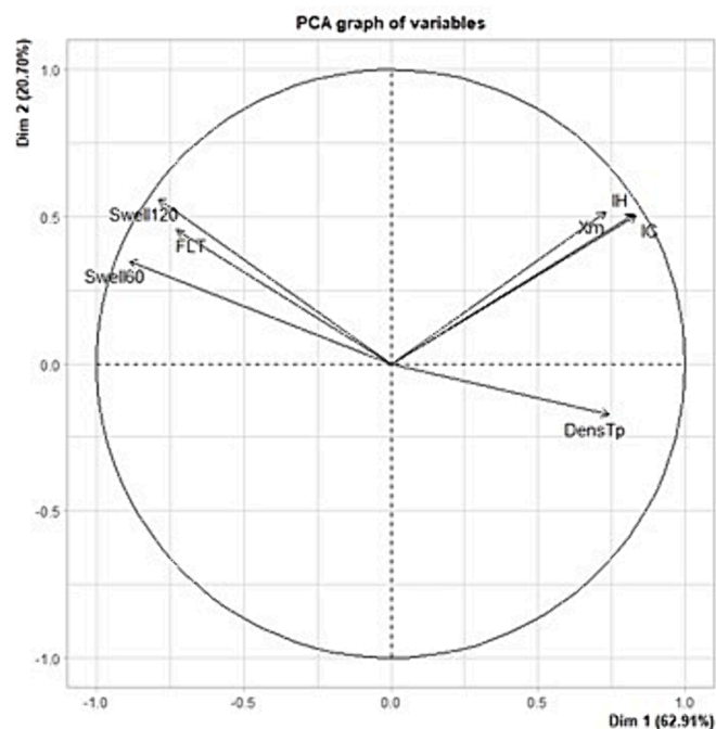
Fig. 1. Loading plot representing the variables direction in the first and second dimensions of PCA. Length of arrows mean influence. Same direction implies correlation. Same direction and sense means positive correlation and same direction and opposite sense indicates negative correlation between variables. Angles close to 90 degrees indicate independence between variables.
