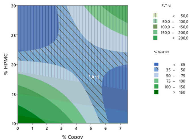
Fig. 5. Superimposed contour plots to delimit the formulation design space. The hold value assigned for % Alginate was 0 for the statistical study. Optimized formula A11 is drawn in the graph.
