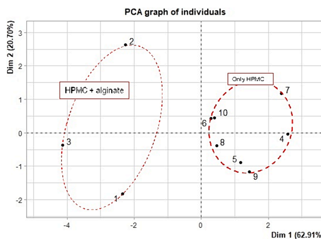
Fig. 2. Score plot representing the formulations in the first and second dimensions of PCA. Relative distance and position mean similarity in formulations. In this figure, two clusters are shown corresponding to only HPMC (right) or HPMC+alginate (left).
