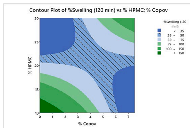
Fig. 4. Contour plot of Swell120 (%) versus %HPMC and %copovidone. The striped area represents the space to achieve a desirable 35–50 % of matrix swelling.
