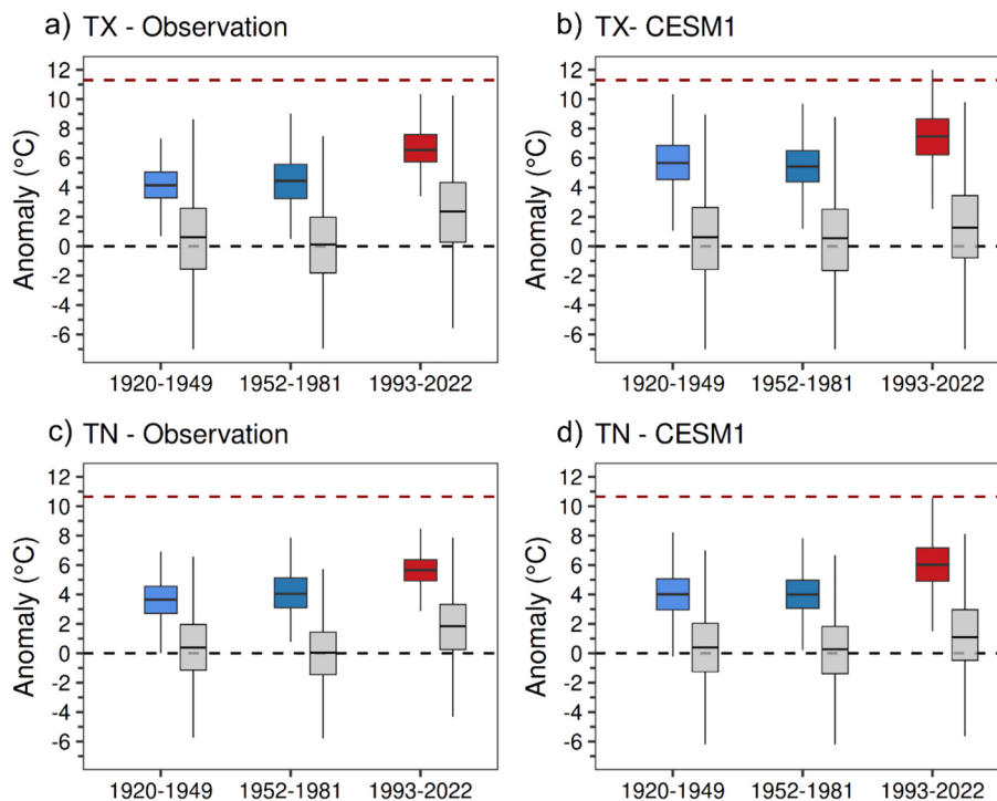
Fig. 3. The distribution of the 3-day mean maximum (a-b, TXm3) and minimum (c-d, TNm3) temperature anomalies for flow analog events (analogs, colored) generated using daily 500 hPa geopotential height from 21 to 23 August and randomly picked days (control, grey) using an in-situ time series (a-c) and CESM1 simulations (b-d). The red dashed horizontal line indicates the maximum (minimum) temperature anomalies of the average of 21–23 August 2023 from the observed time series. Boxes show the 25th–75th percentile ranges and whiskers span the 1st–99th percentiles. (For interpretation of the references to colour in this figure legend, the reader is referred to the web version of this article.)
