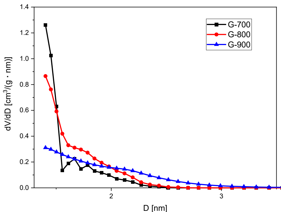
Figure 2. Pore size distribution of ACs calculated from N 2 adsorption.
