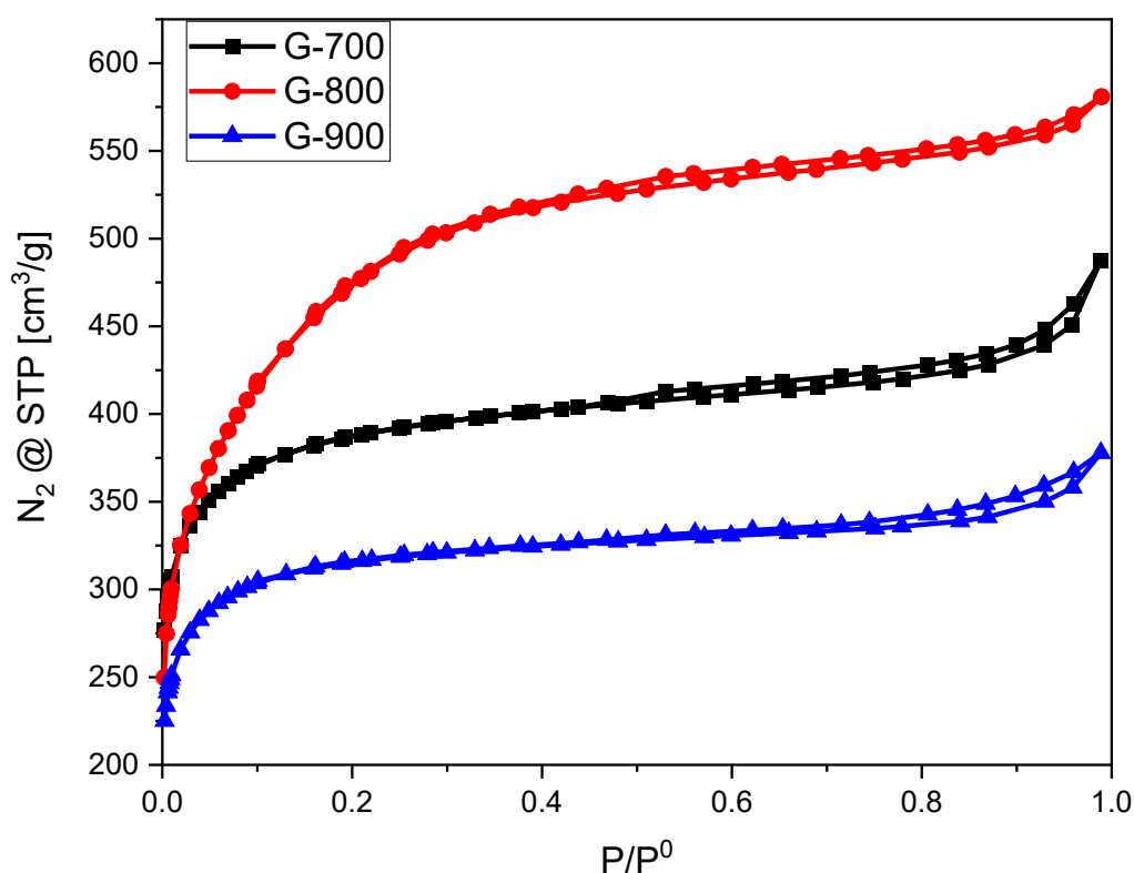
Figure 1. Nitrogen adsorption-desorption isotherms of ACs produced from common fern.
