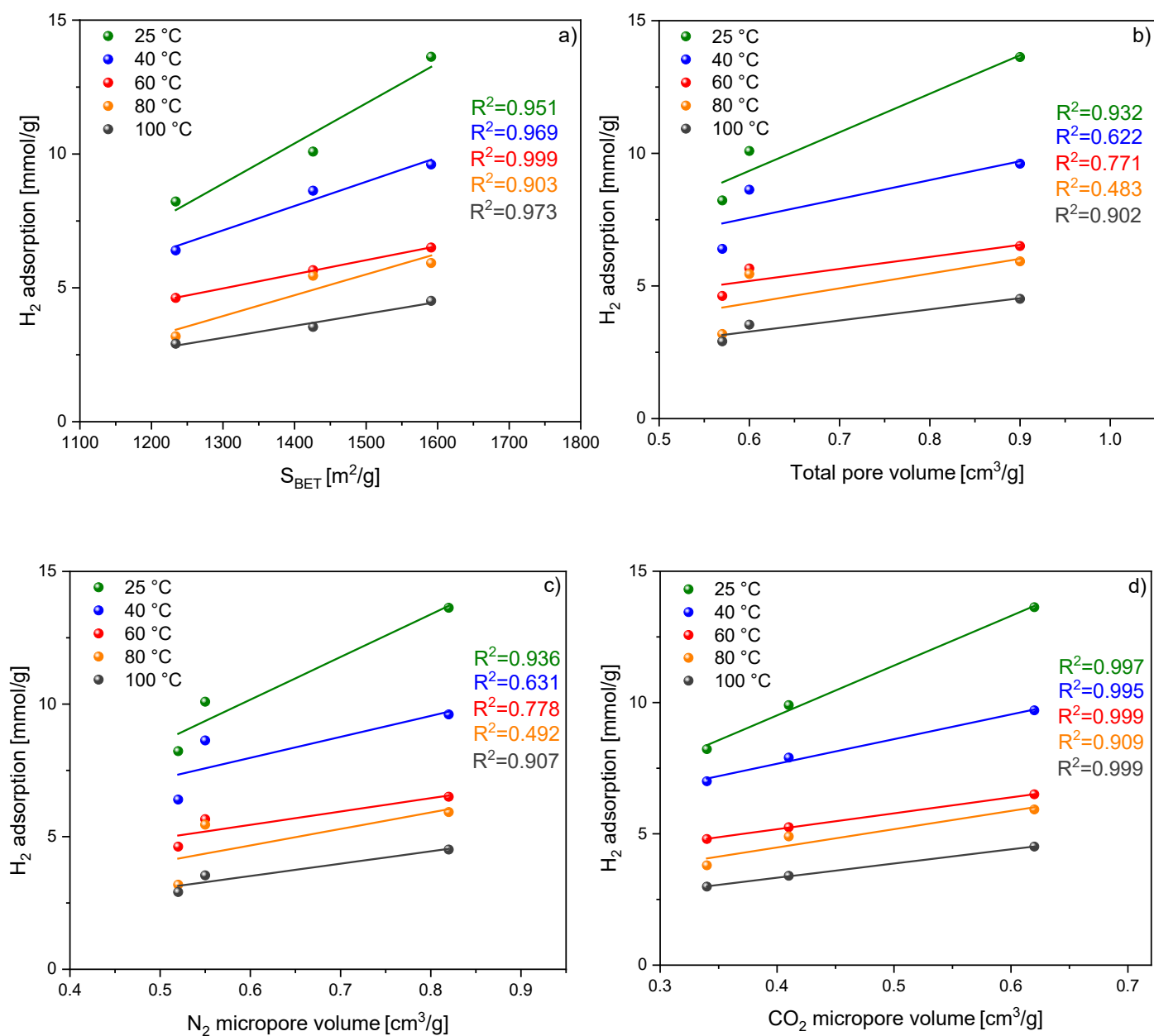
Figure 10. Relationship between different textural parameters and the amount of H 2 adsorbed at 25 °C, 40 °C, 60 °C, 80 °C and 100 °C and 45 bar.
