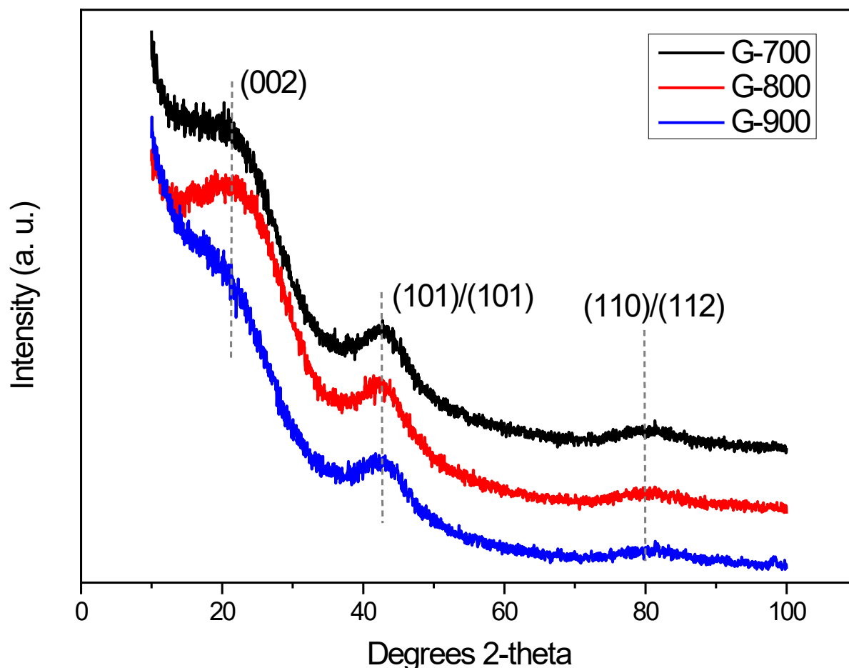
Figure 4. XRD analysis of ACs prepared at different temperatures.
