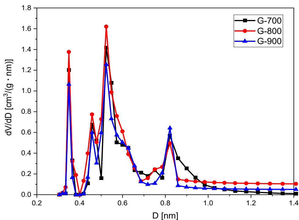
Figure 3. Micropore size distribution of ACs calculated from CO 2 adsorption.
