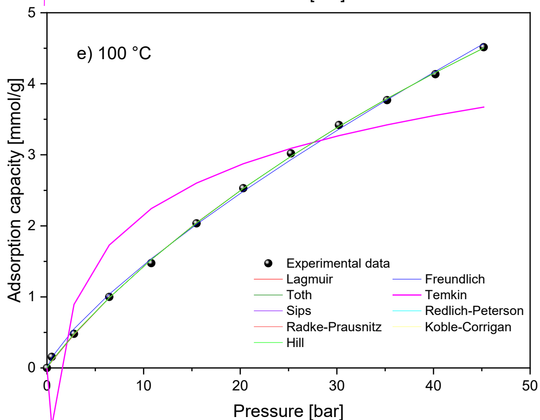
Figure 11. Fitting of H 2 adsorption isotherms to selected models for G-800 at a) 25 °C, b) 40 °C, c) 60 °C, d) 80 °C and e) 100 °C.
