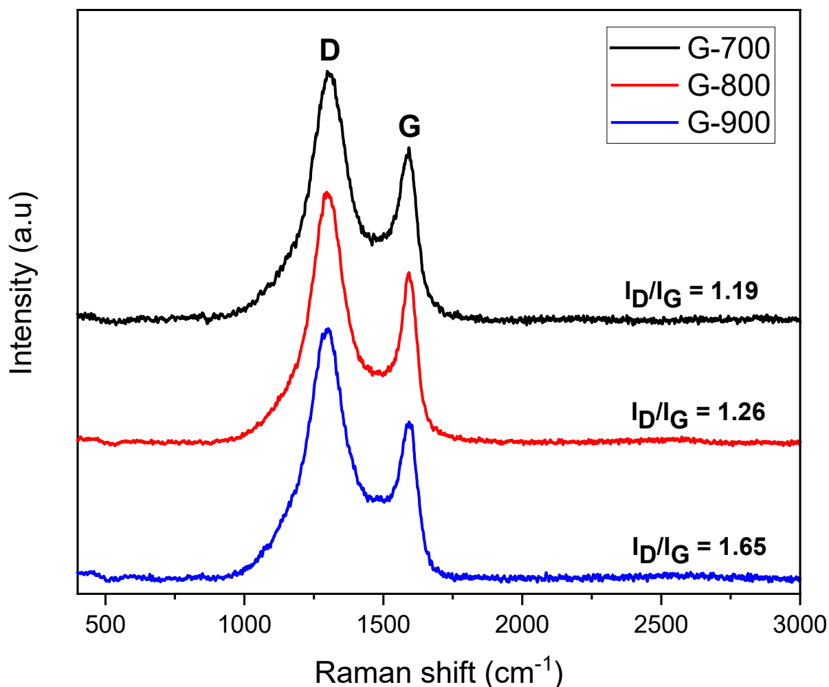
Figure 6. Raman spectra of ACs prepared at different temperatures.
