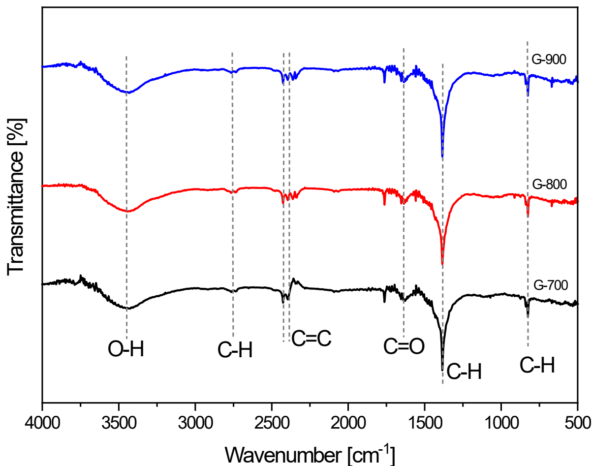
Figure 5. FT-IR spectra of ACs prepared at different temperatures.
