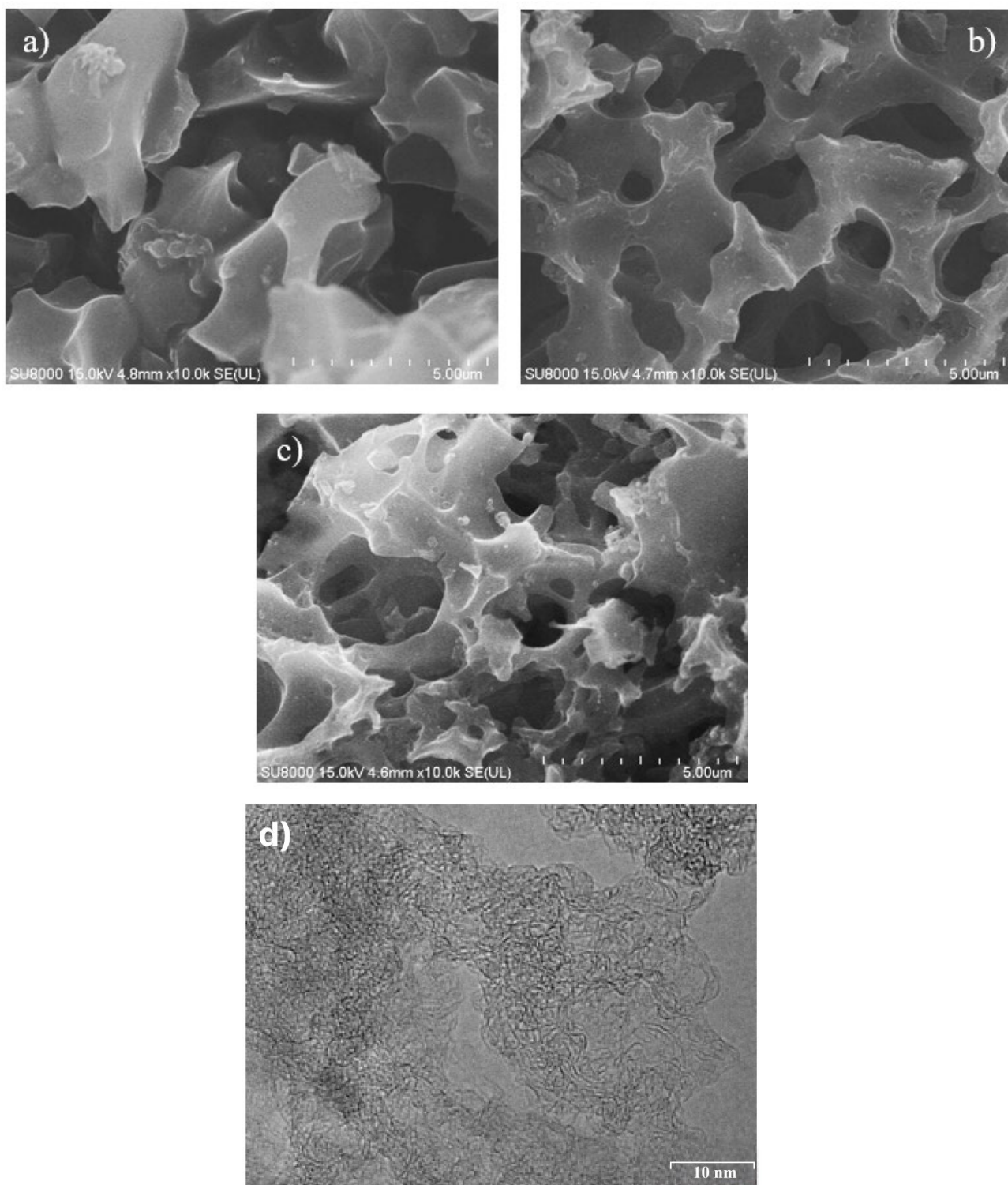
Figure 7. SEM images of ACs prepared at different temperatures: a) G-700; b) G-800 c) G-900 and TEM image of (d) G-800.
