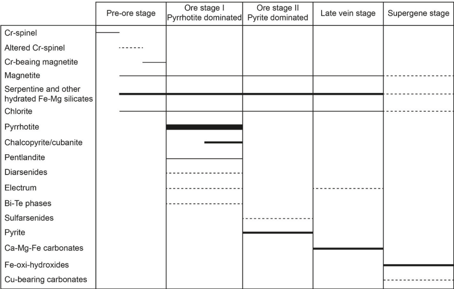
Fig. 13. Paragenetic sequence of the Havana-Matanzas UM-VMS deposits.
