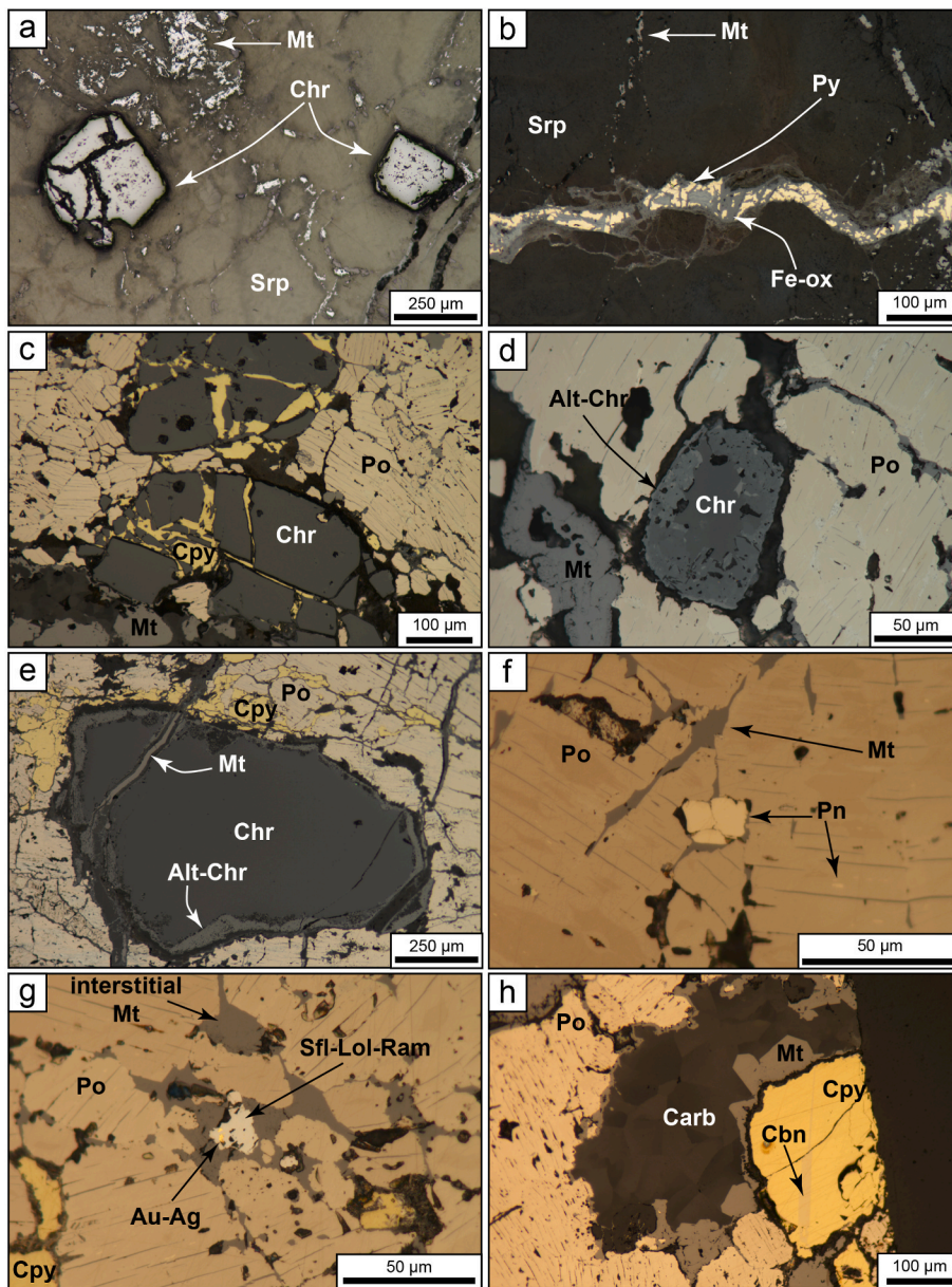
Fig. 4. Optical microscope pictures of a) subhedral Cr-spinel grains from the serpentinite host; b) Pyrite and Fe-oxide vein cutting the serpentinite; c) anhedral and fractured Cr-spinel grains. The fractures are filled with chalcopyrite; d) Cr-spinel grain with alteration rim of porous Cr-spinel; e) large grain of Cr-spinel with a thin rim of altered Cr-spinel crosscut by a late magnetite vein; f) pentlandite grain in an intergranular position with pyrrhotite; g) diarsenide grain from the safflorite-löllingite-rammelsbergite solid solution series with micro-inclusions of electrum; h) late pocket filled with magnetite and carbonates. Abbreviations: alt-chr: altered Cr-spinel, Au-Ag: electrum, carb: carbonates, cbn: cubanite, chr: Cr-spinel, cpy: chalcopyrite, Fe-ox: Fe-oxides, mt: magnetite, pn: pentlandite, po: pyrrhotite, py: pyrite, sfl-lol-ram: safflorite-löllingite-rammelsbergite, srp: serpentinite.
