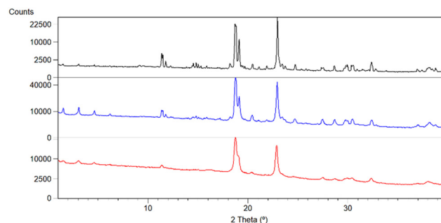
Fig. 5 XRPD comparative diffractograms: in the 1st experiment, heating until 28\text{ °C} (red), in the 2nd experiment, heating until 40\text{ °C} (blue), and ubiquinone bulk powder (black) (see also Fig. S4† for further details).
