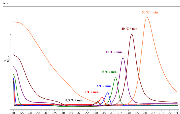
Fig. 2 Overlapping DSC thermograms of ubiquinone after quenching from the melt, from -100\text{ °C} to 0\text{ °C} at different heating rates ( 0.5 , 1 , 2 , 5 , 10 , 20 , and 50\text{ °C min}^{-1} ) (method B, step 3).
