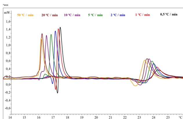
Fig. 3 Overlapping DSC thermograms of ubiquinone at a heating rate of 1\text{ °C min}^{-1} from 0\text{ °C} to 70\text{ °C} (method B, step 4). The heating rates of the previous cold crystallization step (Fig. 2) are shown in the figure for clarity. Enlarged view from 14\text{ °C} to 26\text{ °C} .
