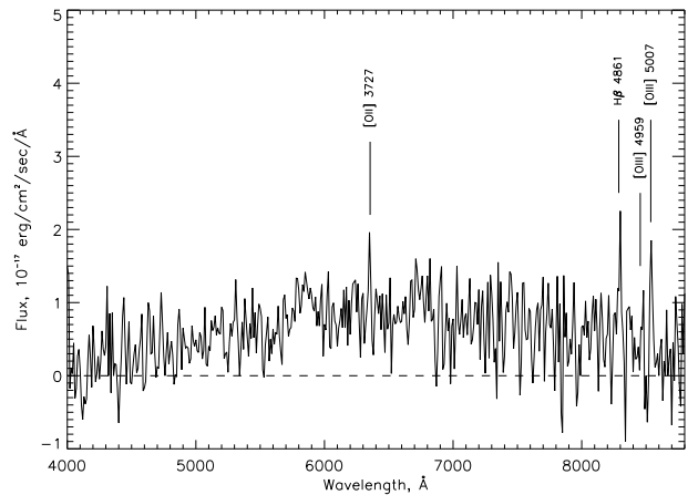
Fig. 5. The BTA/MPSF optical 4500-s spectrum of the GRB 991208 afterglow (on Dec 14.14, 1999 UT) in the 4000 - 8800 Å spectral range. The spectrum has been boxcar smoothed with a 10 Å window. The detection of the four emission lines led to a redshift of z = 0.7063 \pm 0.0017 , that of the host galaxy.
