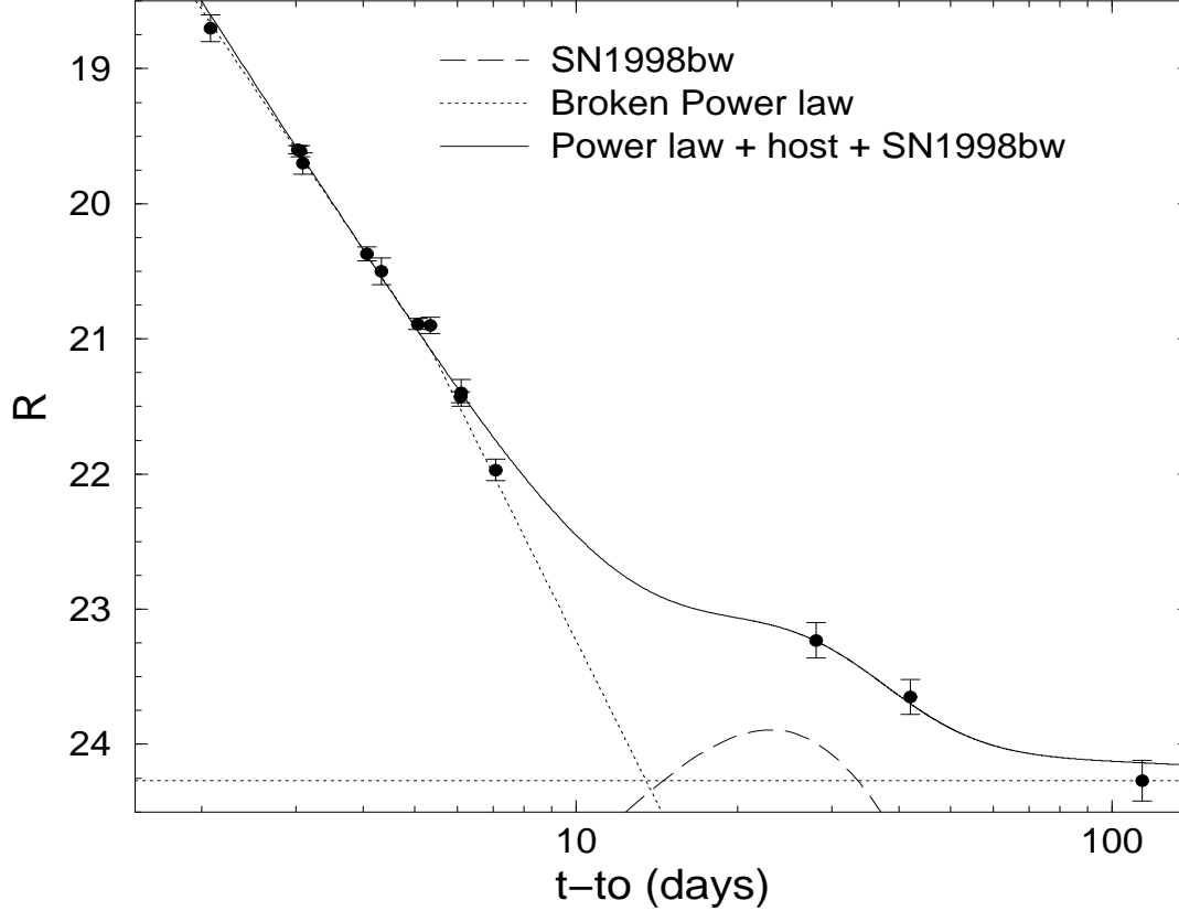
Fig. 4. The GRB 991208 R-band light curve (solid line) fitted with a SN1998 bw-like component at z = 0.706 (long dashed line) superposed to the broken power-law OA light curve displaying the second break at t_{break} \sim 5 d (with \alpha_1 = -2.3 and \alpha_2 = -3.2 , short dotted lines) and the constant contribution of the host galaxy ( R = 24.27 \pm 0.15 , dotted line).
