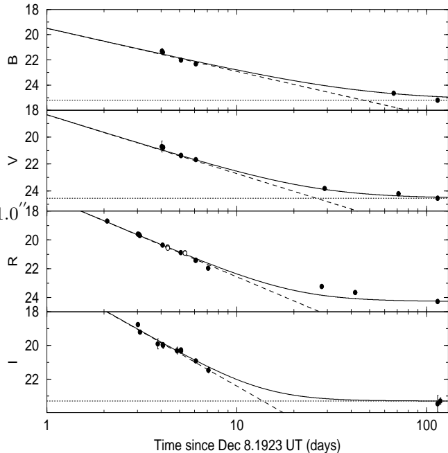
Fig. 2. The BVRI -band light-curves of the optical transient related to GRB 991208, including the underlying galaxy. Filled circles are our data, empty circles are data from Garnavich and Noriega-Crespo (1999) and Halpern and Helfand (1999). The dashed-line is the pure OA contribution to the total flux, according to the single power-law fits given on Table 2. The dotted line is the contribution of the host galaxy. The solid line is the combined flux (OA plus underlying galaxy).
