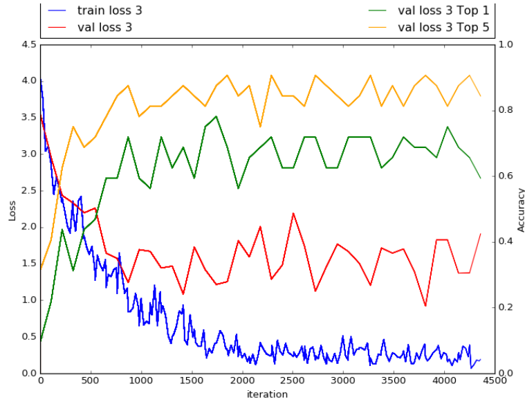
Figure 2.14: GoogLeNet Train and Validation loss, Validation Top 1 and Top5
