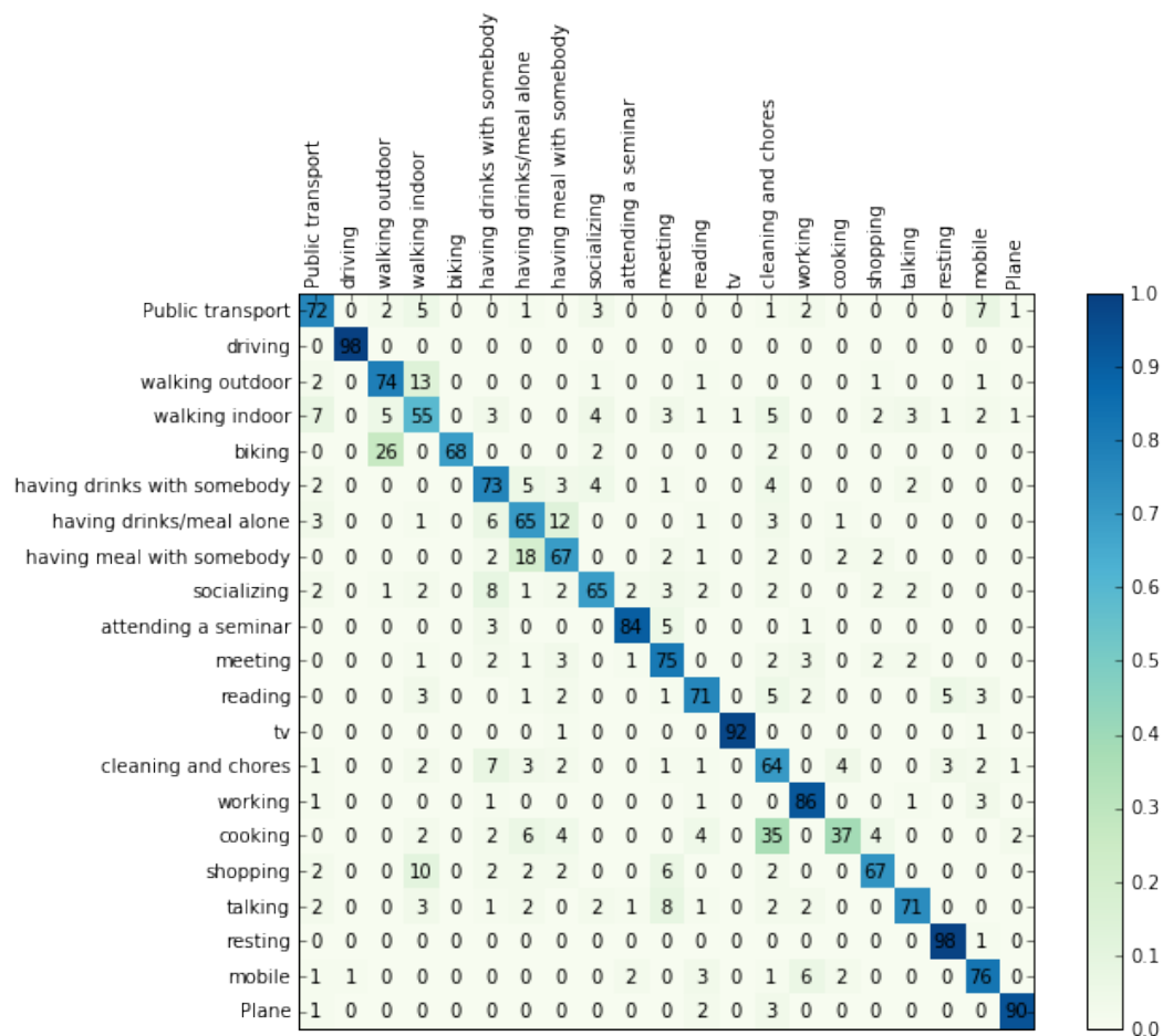
Figure B.4: Confusion matrix for finetuned GoogLeNet + RDF. Columns are the predicted labels and rows the real labels
