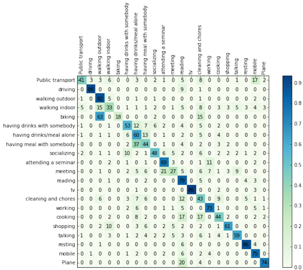
Figure B.2: Confusion matrix for finetuned GoogLeNet. Columns are the predicted labels and rows the real labels
