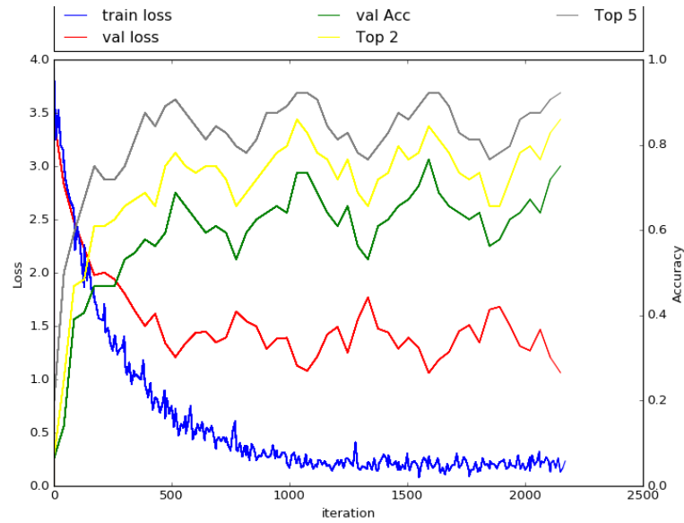
Figure 2.12: AlexNet Train loss, Validation loss and Validation accuracy Top 1, 2 and 5
