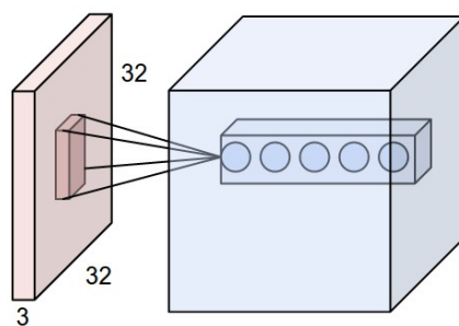
Figure 2.9: Output volume and depth column representation a
