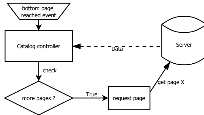
Figure 1.10: How a new set of pictures is loaded
