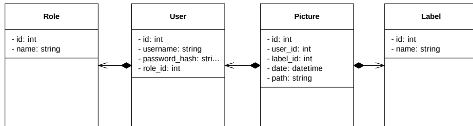
Figure 1.4: A representation of the data
