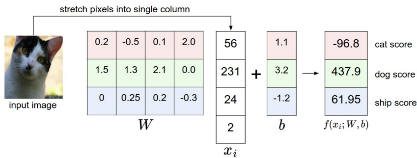
Figure 2.3: Example of classifying from an input image to a class a
