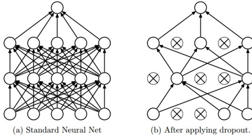
Figure 2.8: An example of applying dropout to a network a
