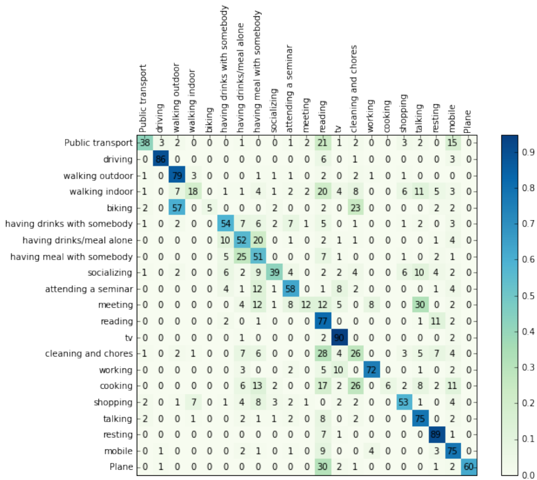
Figure B.1: Confusion matrix for finetuned AlexNet. Columns are the predicted labels and rows the real labels
