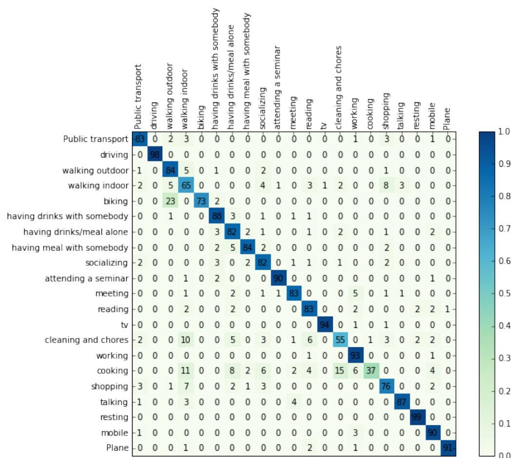
Figure B.6: Confusion matrix for finetuned AlexNet + RDF for layers FC7 and probs. Columns are the predicted labels and rows the real labels
