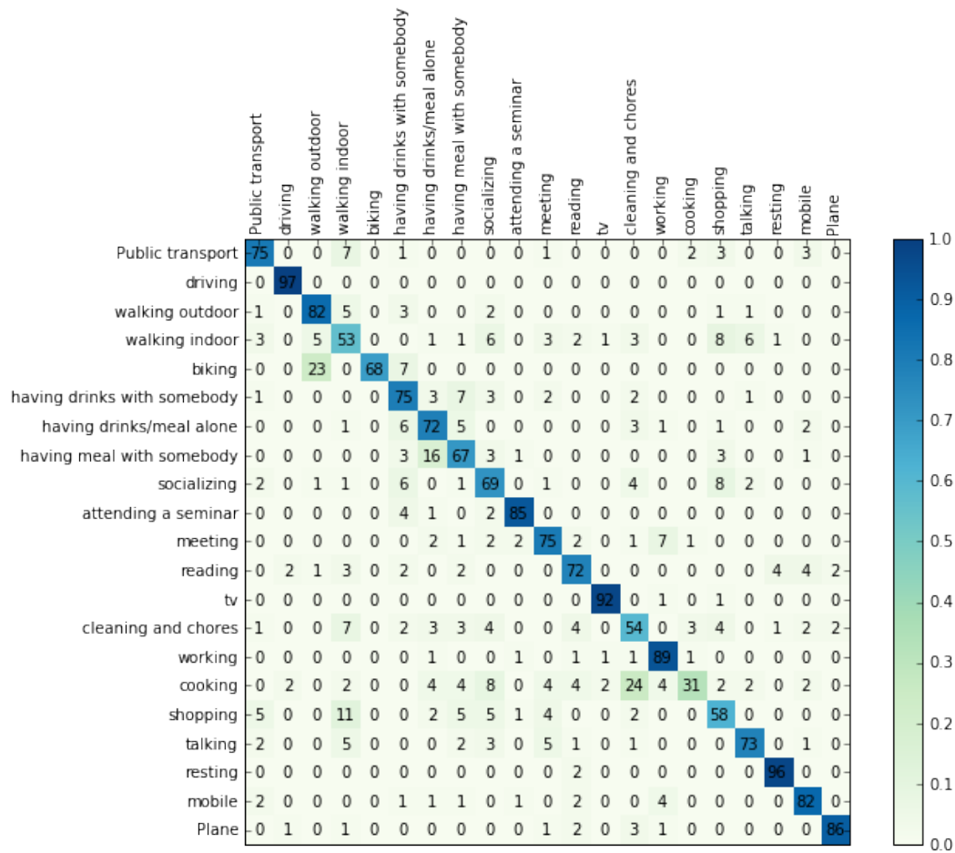
Figure B.3: Confusion matrix for finetuned AlexNet + RDF. Columns are the predicted labels and rows the real labels
