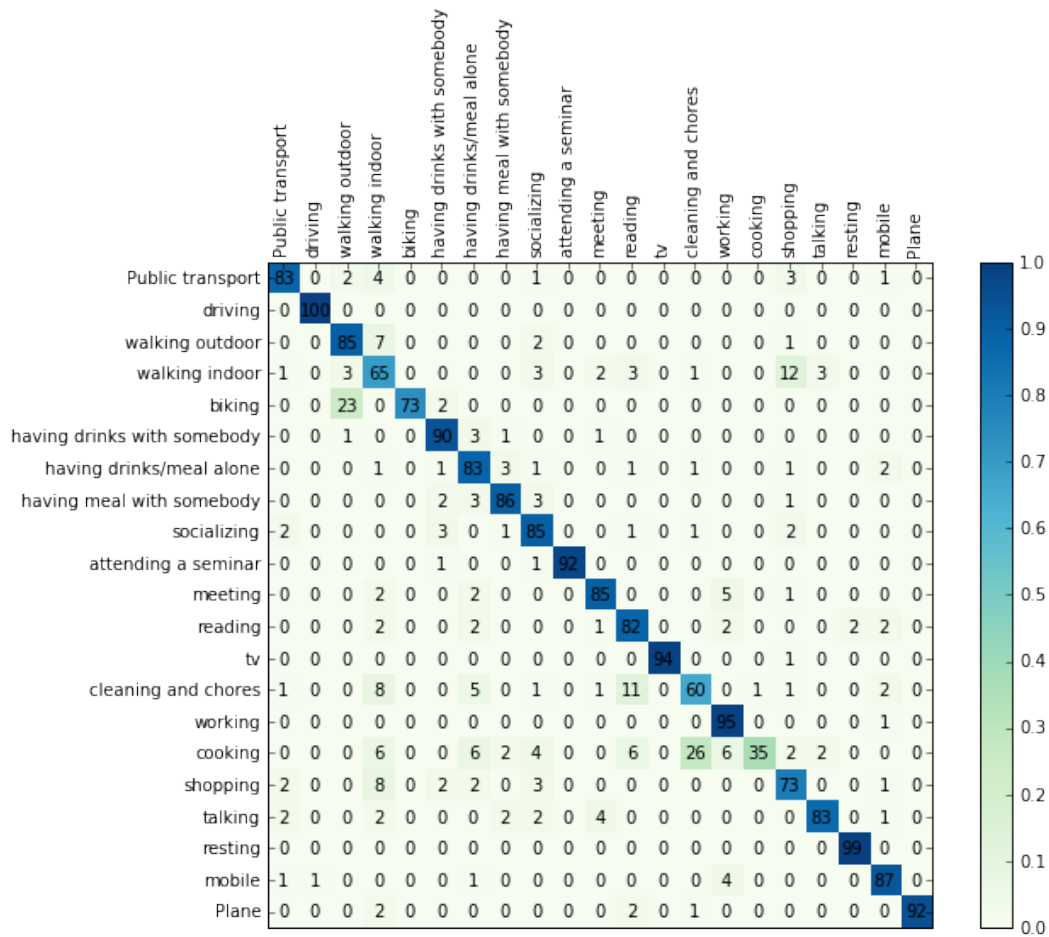
Figure B.5: Confusion matrix for finetuned AlexNet + RDF for layers FC6 and probs. Columns are the predicted labels and rows the real labels
