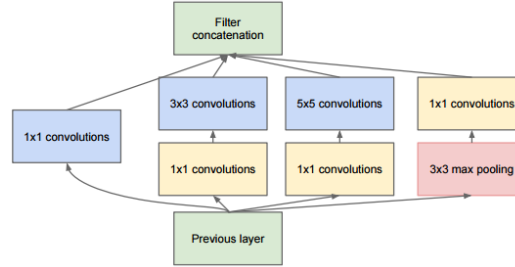
Figure 2.11: Inception module with dimensionality reduction a
