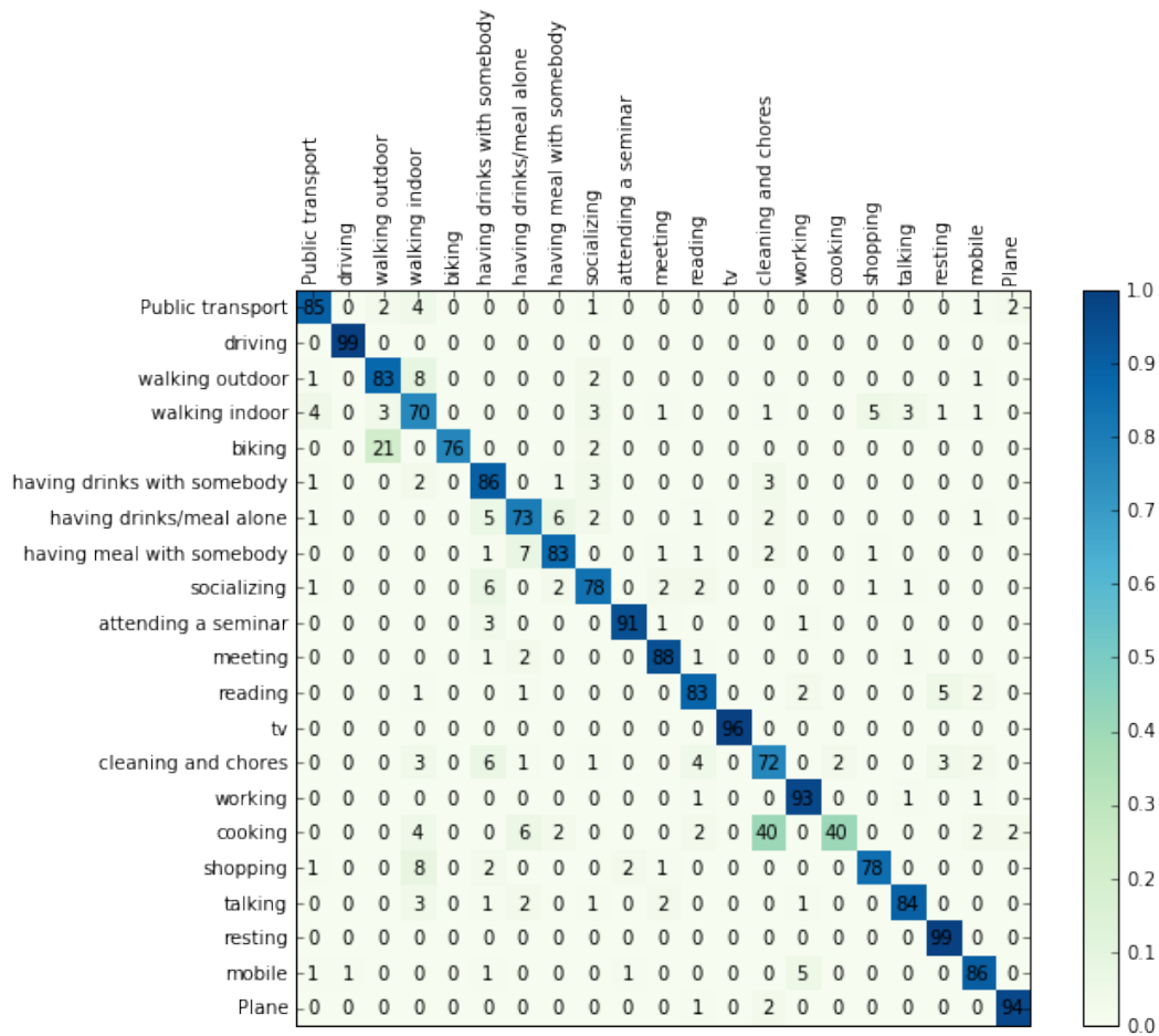
Figure B.7: Confusion matrix for finetuned GoogLeNet + RDF for layers Pool5 and probs. Columns are the predicted labels and rows the real labels
