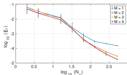
Figure 9. (Left) Logarithm of the mean relative energy error E_r as a function of the logarithm of the number of sampling points N_e and for different number of excited CWFs M = \{1, 2, 3, 4\} . Error bars represent the standard deviation of the relative error.
