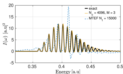
Figure 3. S 2 ← S 0 spectra of ICWF-kick (gold) and multitrajectory Ehrenfest \delta -kick (MTEF-kick) (blue) compared to the exact peak placement overlaid as a black line, showing that while mean-field theory is unable to capture qualitatively the correct vibronic line shape spacing and intensity, the sta-ICWF approach accurately captures the exact spectrum.
