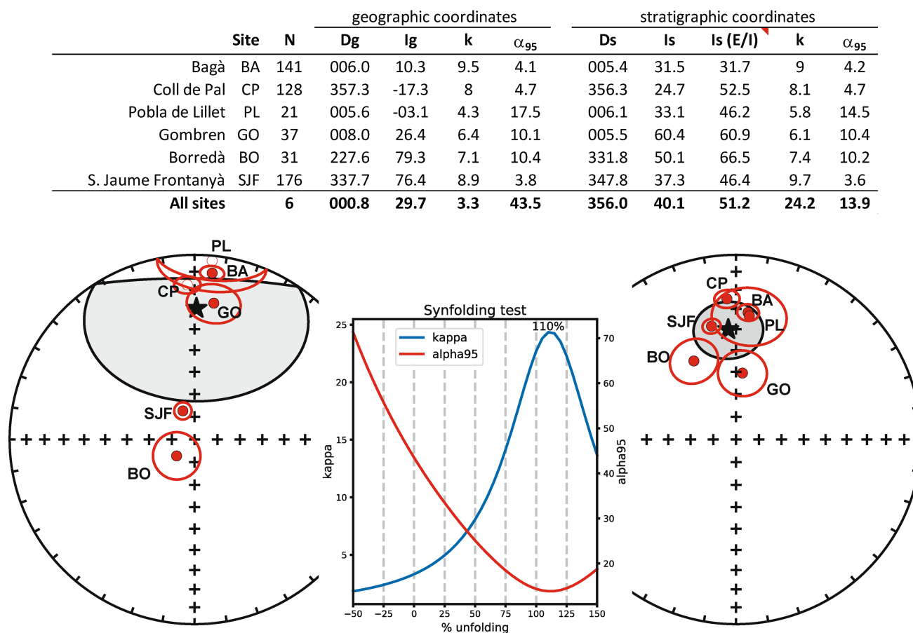
FIGURE 5 Mean palaeomagnetic directions and Fisher statistics at section level and the overall mean in geographic and (tilt-corrected) stratigraphic coordinates. Mean directions were corrected for inclination error using the E/I method of Tauxe et al. (2008). Stepwise unfolding yielded best kappa and \alpha_{95} Fisher parameters after 110% unfolding (see text for discussion).
